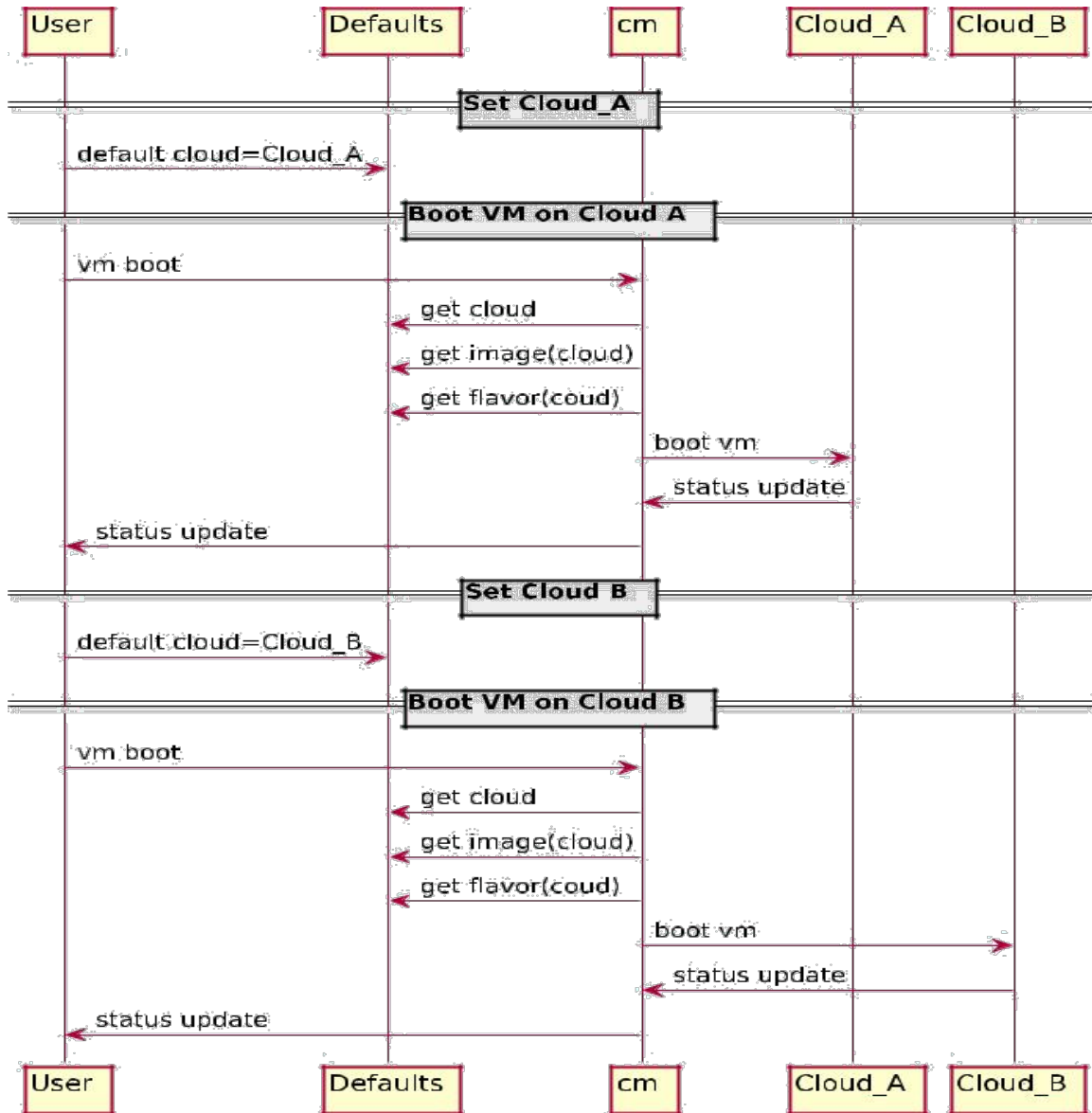
Figure 3: Booting a VM from Defaults
