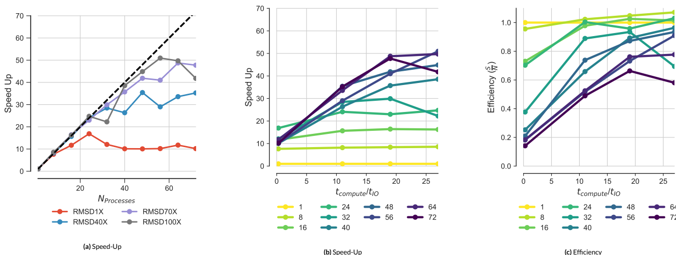
FIGURE B4 Effect of R_{\text{comp}/\text{IO}} ratio on performance of the RMSD task on SDSC Comet . We tested performance for R_{\text{comp}/\text{IO}} ratios of 0.3, 11, 19, 27, which correspond to 1 \times \text{RMSD} , 40 \times \text{RMSD} , 70 \times \text{RMSD} , and 100 \times \text{RMSD} respectively. (a) Effect of R_{\text{comp}/\text{IO}} on the speed-up. (b) Change in speed-up with respect to R_{\text{comp}/\text{IO}} for different processor counts. (c) Change in the efficiency with respect to R_{\text{comp}/\text{IO}} for different processor counts.
