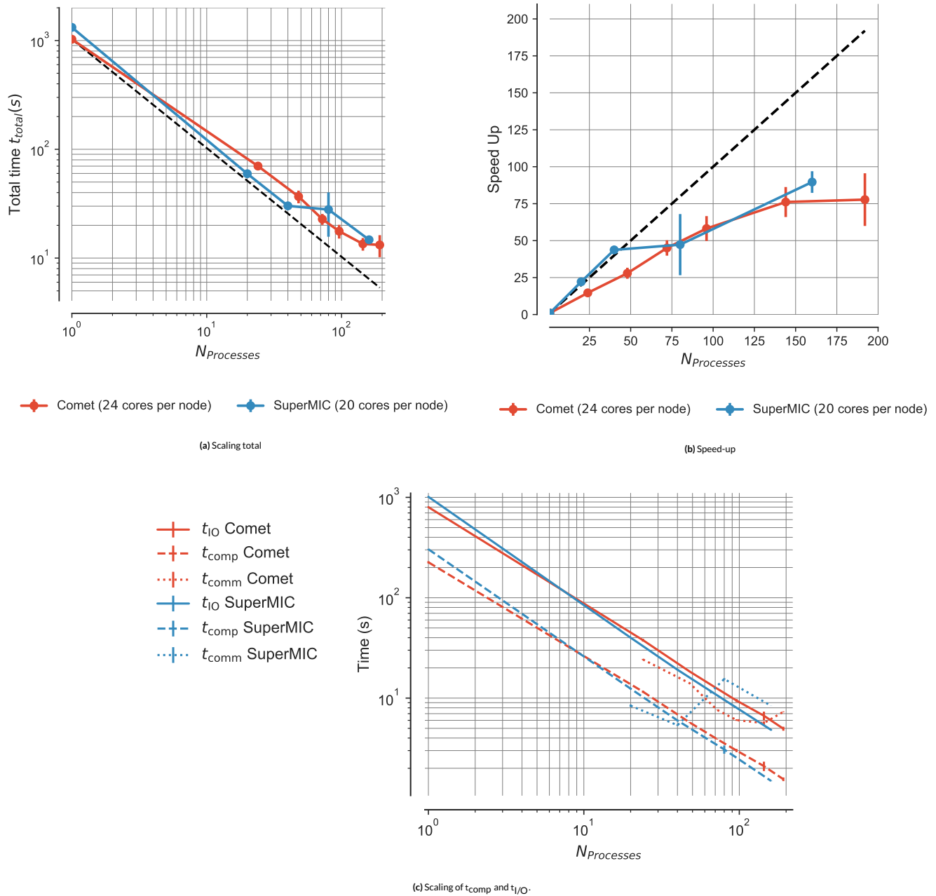
FIGURE 6 Comparison of the performance of the RMSD task across different clusters [SDSC Comet (24 cores per node), LSU SuperMIC (20 cores per node)] when the trajectories are split (subfiling). Five repeats were performed to collect statistics. The error bars show the standard deviation with respect to the mean.
