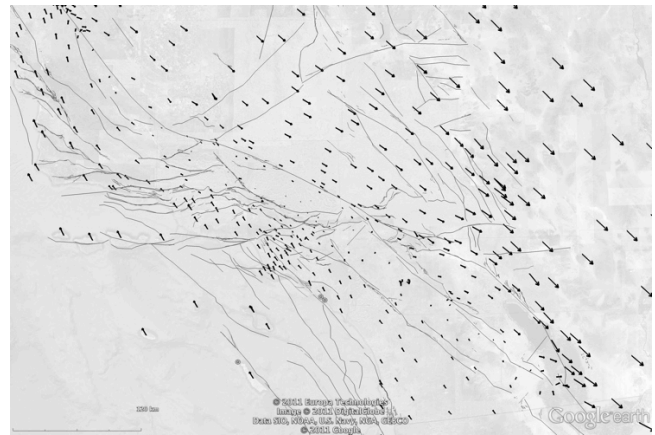
Figure 6. GPS vectors plotted for southern California relative to station CHIL in the San Gabriel Mountains. Fault traces are from UCERF-2 [4].
