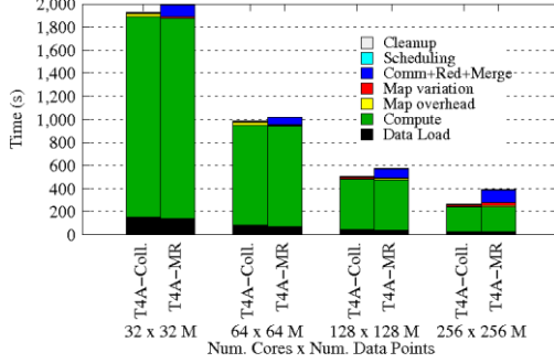
Figure 12. K-means Clustering strong scaling. 500 Centroids, 20 Dimensions, 10 iterations. 128Million data points.
