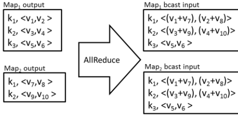
Figure 4. Example Map-AllReduce with Sum operation
