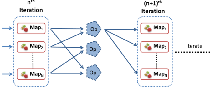
Figure 3. Map-AllReduce collective
