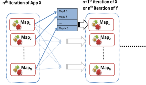
Figure 2. Map-AllGather Collective
