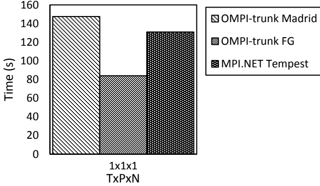
Fig. 14 DAVS Charge6 performance on single node
