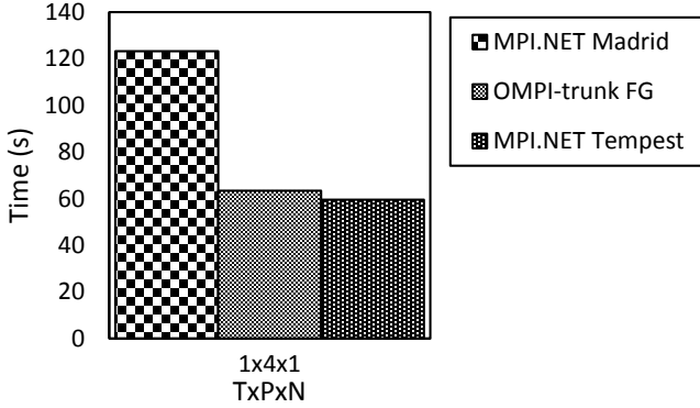
Fig. 15 DAVS Charge6 performance on single node with multiple processes
