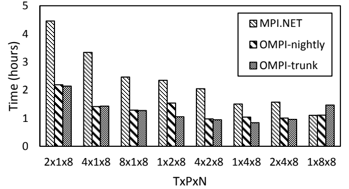
Fig. 11 DAVS Charge2 performance with threads
