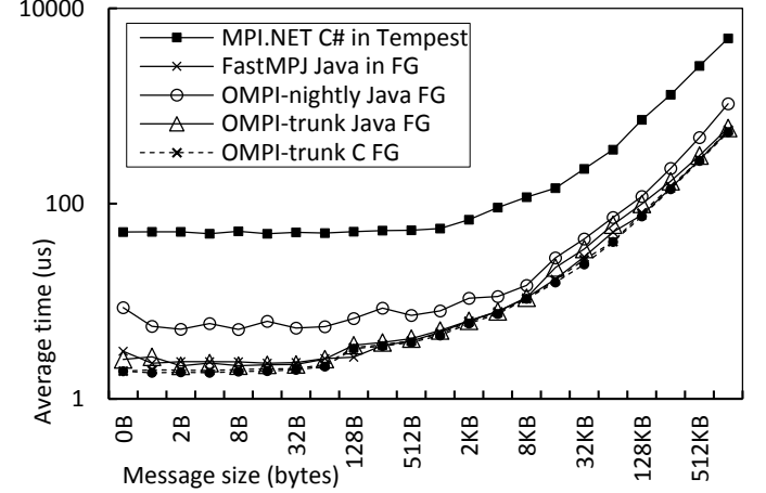
Fig. 4 Performance of MPI send and receive operations
