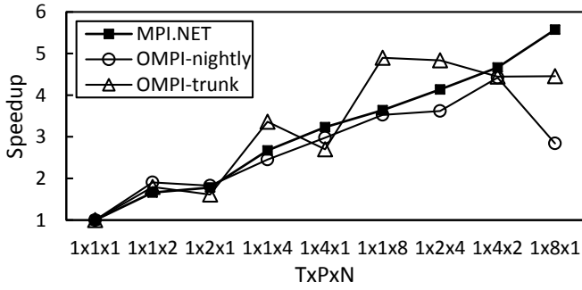
Fig. 8 DAVS Charge5 speedup
