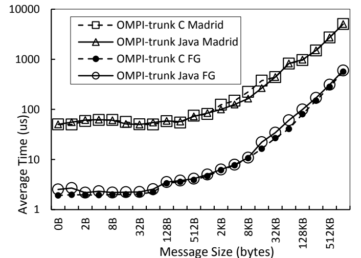
Fig. 6 Performance of MPI send and receive on Infiniband and Ethernet
