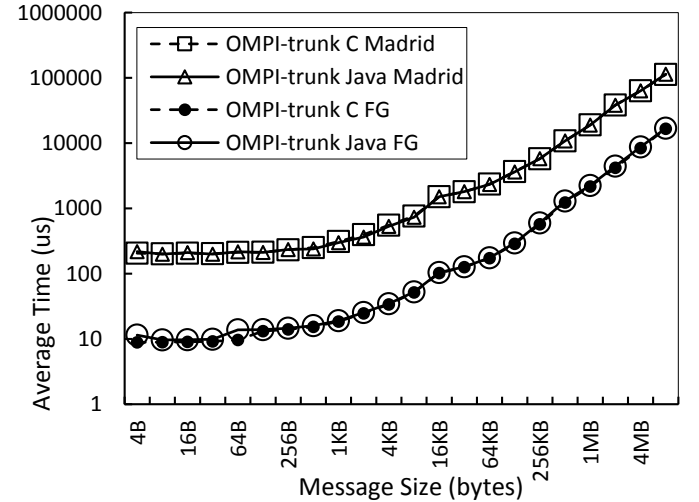
Fig. 5 Performance of MPI allreduce on Infiniband and Ethernet
