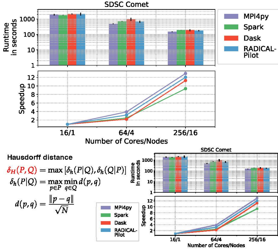
Figure 4-4 Path similarity analysis with the Hausdorff distance \delta_H(P, Q) between trajectories P and Q , consisting of coordinate frames p and q . Strong scaling was studied for 4 different frameworks on SDSC XSEDE facility Comet for N=128 trajectories resulting in 8128 Hausdorff distance calculations.[76]
