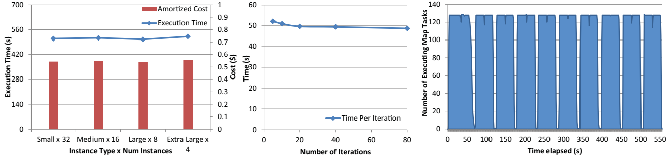
Figure 4. Twister4Azure KMeansClustering (20D data with 500 centroids, 32 cores). Left(a) : Instance type study with 10 iterations 32 million data points. Center(b) : Time per iteration with increasing number of iterations 32 million data points.
