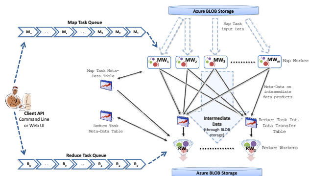
Figure 1. MRRoles4Azure Architecture[1]
