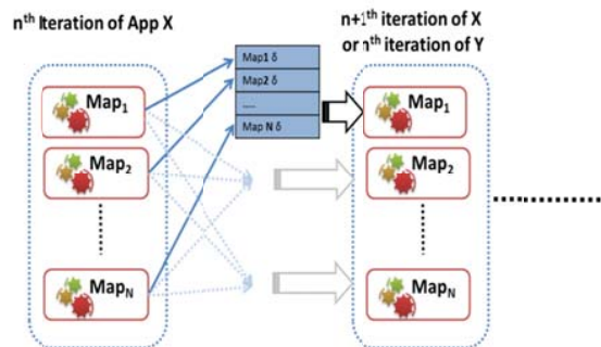
Figure 2. Map-AllGather Collective
