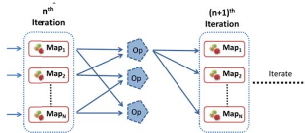
Figure 3. Map-AllReduce collective
