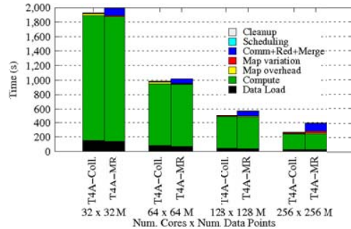
Figure 12. Twister4Azure K-means Clustering strong scaling. 500 Centroids, 20 Dimensions, 10 iterations. 128 million data points.
