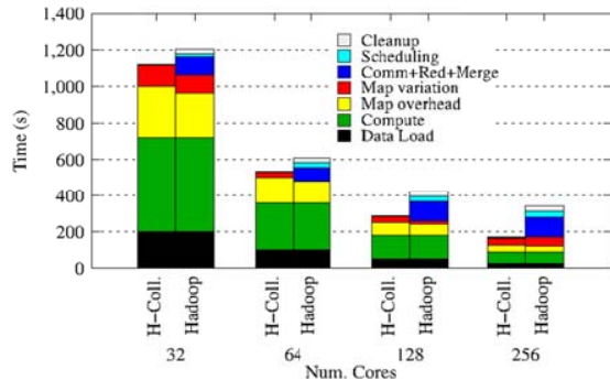
Figure 10. Hadoop MapReduce K-means Clustering & H-Collectives Map-AllReduce Strong scaling. 500 Centroids, 20 Dimensions, 10 iterations.
