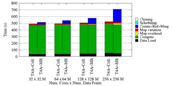
Figure 11. Twister4Azure K-means weak scaling with Map-AllReduce. 500 Centroids, 20 Dimensions. 10 iterations. 32 to 256 Million data points.
