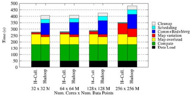
Figure 9. Hadoop K-means Clustering comparison with H-Collectives Map-AllReduce Weak scaling. 500 Centroids, 20 Dimensions, 10 iterations.
