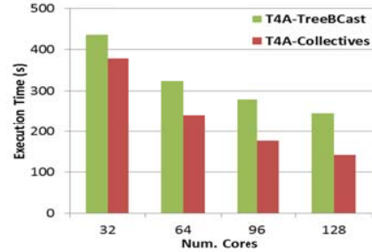
Figure 6. MDS application implemented using Twister4Azure. 20 iterations. 51,200 data points (~5GB).
