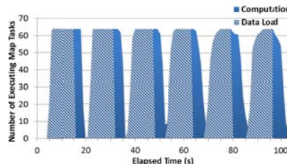
Figure 8. H-Collectives AllGather MDS-BCCalc histogram
