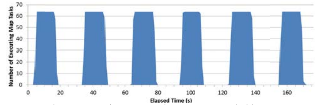
Figure 7. Hadoop MapReduce MDS-BCCalc histogram
