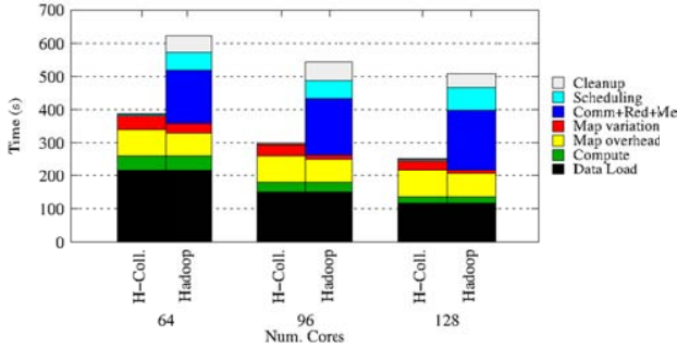
Figure 5. MDS Hadoop using only the BC Calculation MapReduce job per iteration to highlight the overhead. 20 iterations, 51,200 data points.
