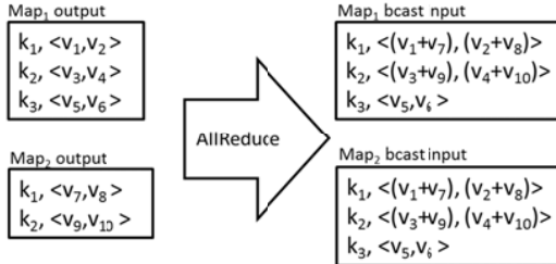
Figure 4. Example Map-AllReduce with Sum operation
