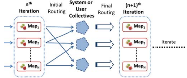
Figure 1. Map-Collective primitives
