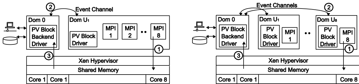
Figure 16. Communication between dom0 and domU when 1-VM per node is deployed (left). Communication between dom0 and domUs when 8-VMs per node are deployed (right).
