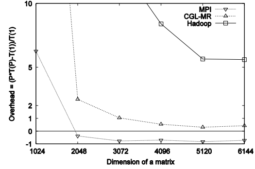
Figure 7. Overhead induced by different parallel programming runtimes for the matrix multiplication application (8 nodes are used)
