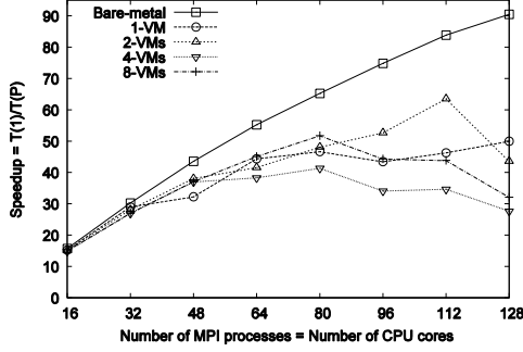
Figure 12. Speed-up of the Kmeans clustering (Number of data points = 860160 )
