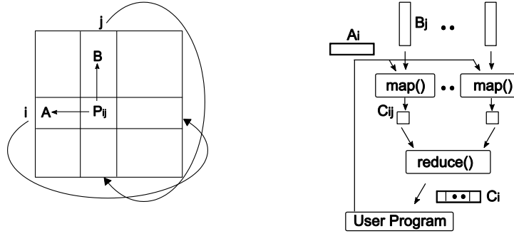
Figure 1. Communication topology of matrix multiplication applications implemented using Cannon's algorithm (left) and MapReduce programming model (right).
