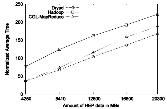
Figure 3. Performance of HEP data analysis applications
