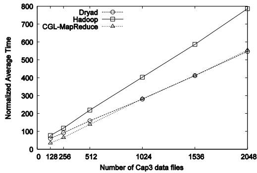
Figure 2. Performance of the Cap3 application
