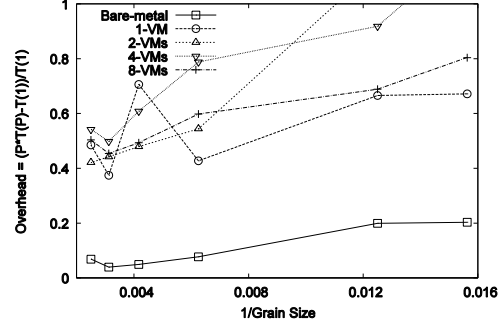
Figure 15. Total overhead of the Concurrent Wave Solver (Number of MPI Processes = 128 )
