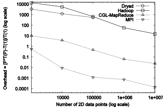
Figure 6. Overhead induced by different parallel programming runtimes for the Kmeans Clustering application (Note: Both axes are in log scale)
