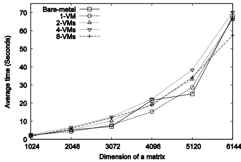
Figure 8. Performance of the matrix multiplication application (Number of MPI processes = 64)
