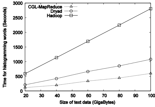
Figure 4. Performance of the Word Histogramming applications
