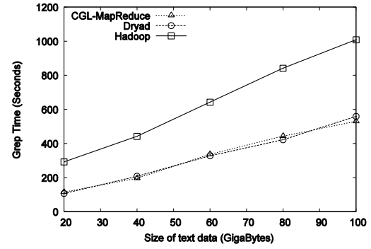
Figure 5. Performance of the Distributed Grep applications
