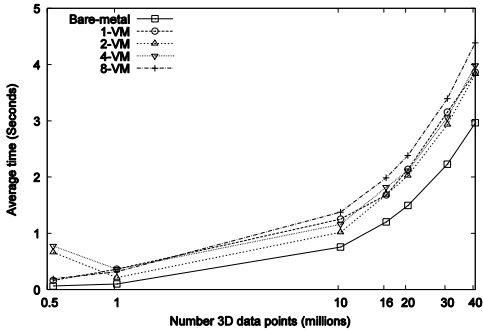
Figure 10. Performance of Kmeans clustering (Number of MPI Processes = 128 )
