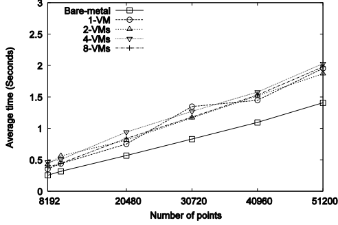
Figure 14. Performance of the Concurrent Wave Solver (Number of MPI Processes = 128 )
