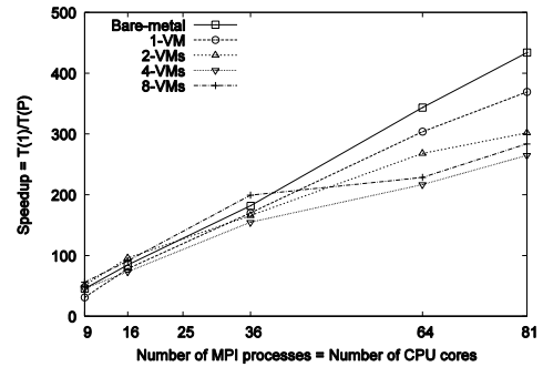
Figure 9. Speed-up of the matrix multiplication application (Matrix size = 5184x5184)
