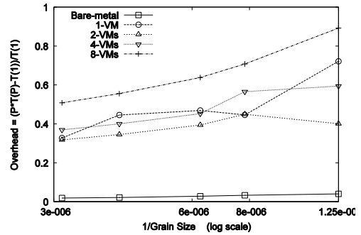
Figure 11. Total overhead of the Kmeans clustering (Number of MPI Processes = 128 )
