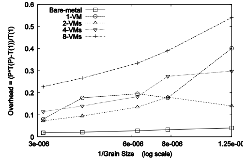
Figure 13. Parallel overhead of the Kmeans clustering (Number of MPI Processes = 128 )
