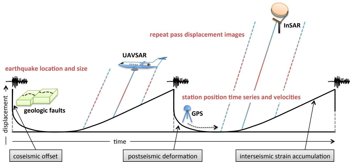
Figure 1. Schematic of earthquake cycle of strain accumulation and release with the long-term tectonic rate removed.
