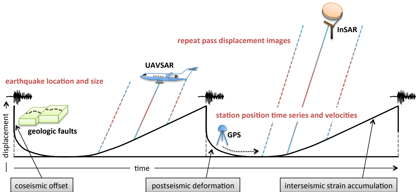
Figure 1. Schematic of the earthquake cycle of strain accumulation and release with the long-term tectonic rate removed.
