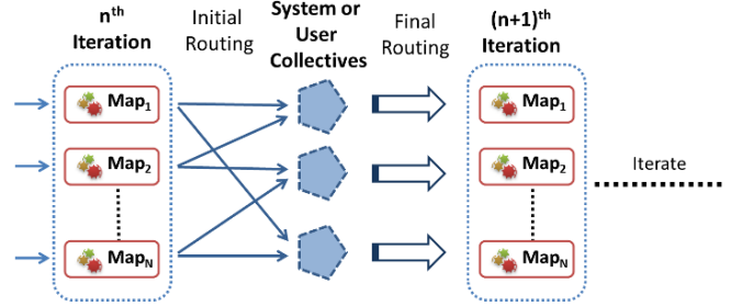
Figure 1. Map-Collective primitives
