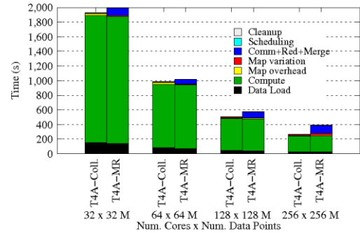
Figure 12. Twister4Azure K-means Clustering strong scaling. 500 Centroids, 20 Dimensions, 10 iterations. 128 Million data points.
