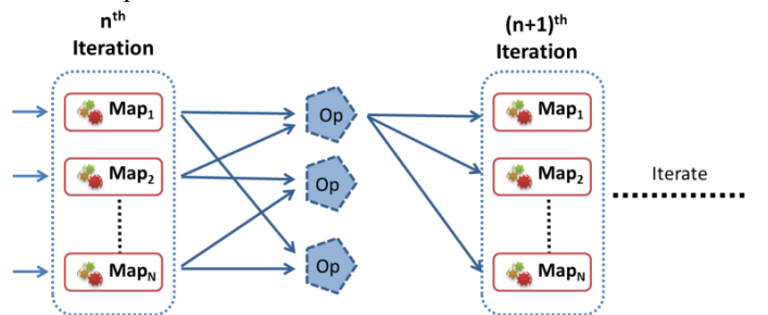
Figure 3. Map-AllReduce collective
