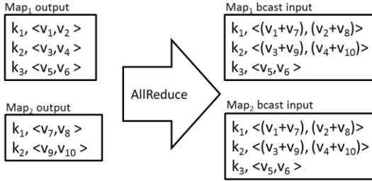
Figure 4. Example Map-AllReduce with Sum operation
