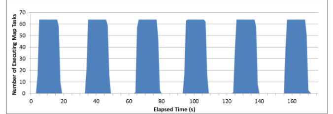
Figure 7. Hadoop MapReduce MDS-BCCalc histogram
