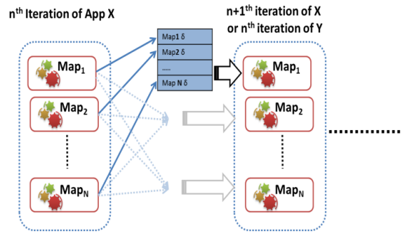
Figure 2. Map-AllGather Collective
