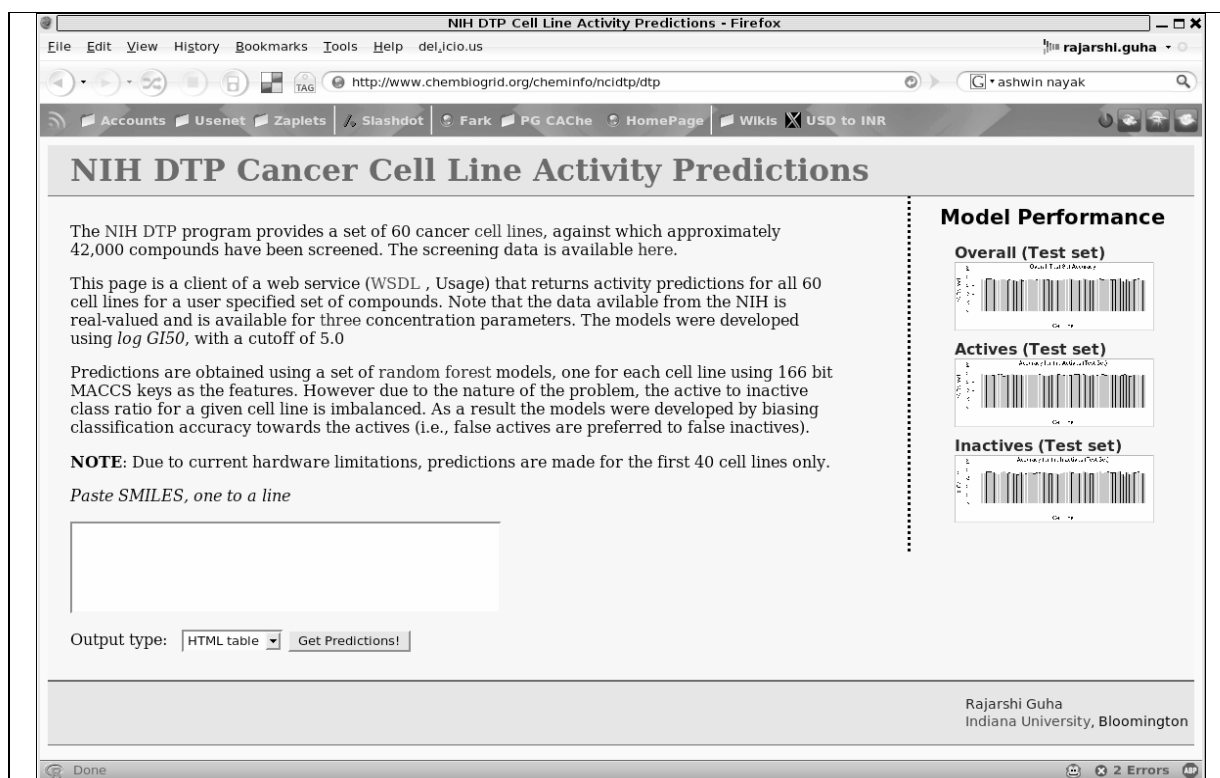
Fig. 2. A screen shot of a web page client that provides access to a set of models that predict the anti-cancer activity of a compound, given its SMILES, against the 60 cancer cell lines hosted by the NIH NCI Developmental Therapeutics Program.
