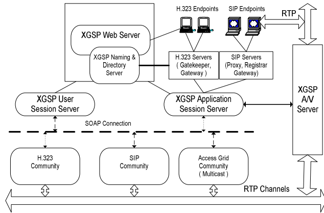
Figure 3 XGSP Prototype Systems
