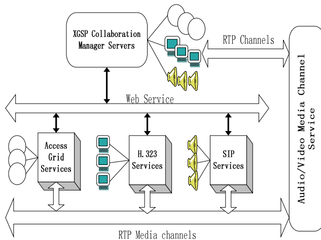
Figure 1 XGSP Conference Control Framework
