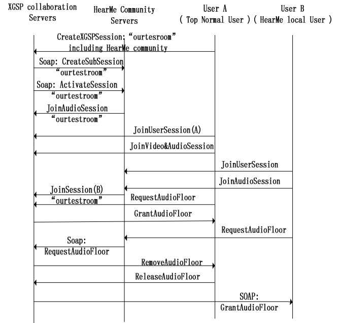
Fig 4 an example of XGSP conference control procedure
