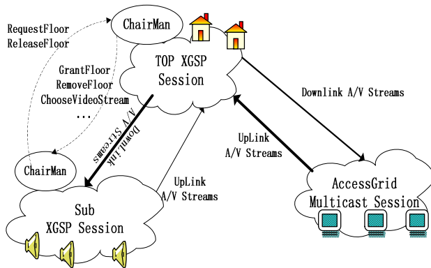
Figure 2 XGSP floor control
