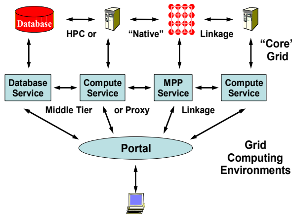
Fig. 1. Middle-Tier and Raw (HPC) Linked Components of an Application showing both the “Core” and Computing Environments
