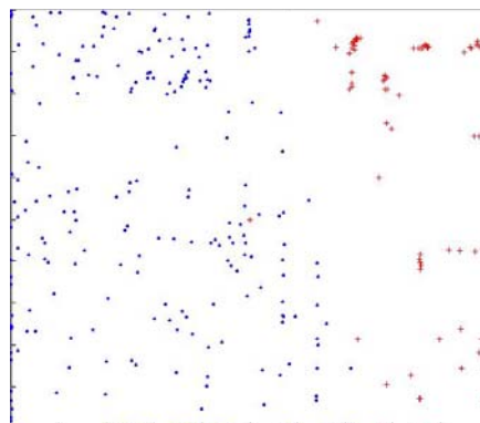
Figure 2. GTM Projection for 2 clusters from DA in space of 155 Chemical Properties labeled as a . or +
