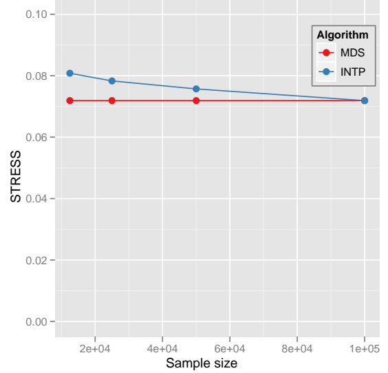
Figure 3: Quality comparison between Interpolated result of 100k with respect to the different sample size (INTP) and 100k MDS result (MDS)
