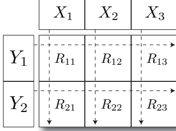
Figure 2: An example of decomposition in GTM interpolation for computing responsibility matrix \mathbf{R} in parallel by using a 2 \times 3 virtual processor grid.
