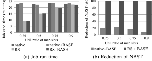
Figure 4. Results of running PSA-SWG
