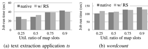
Figure 8. Experiment with IO-intensive workload
