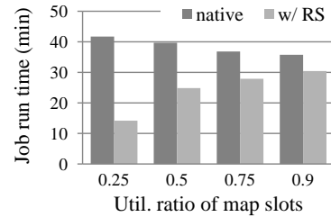
Figure 7. Experiment with network-intensive workload mr-wc
