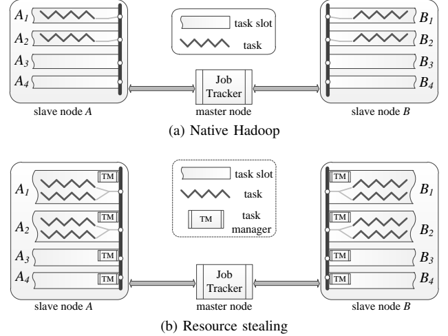
Figure 2. Scheduling with native Hadoop and resource stealing
