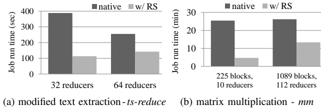
Figure 6. Results for reduce-mostly applications
