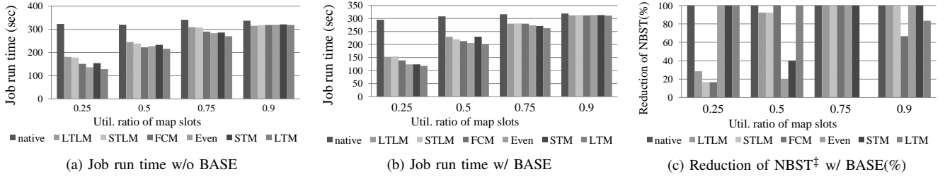
Figure 3. Results of running ts-map ( \dagger NBST: Non-Beneficial Speculative Tasks)
