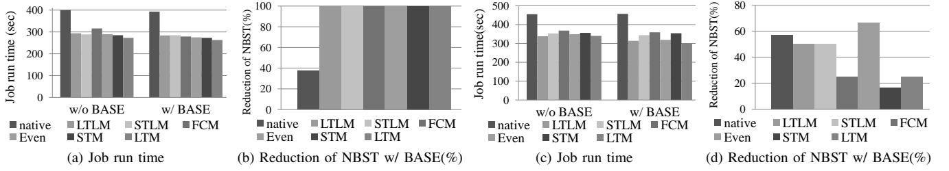
Figure 5. Run ts-map with straggler nodes. There are two straggler nodes for (a) and (b), and four straggler nodes for (c) and (d)
