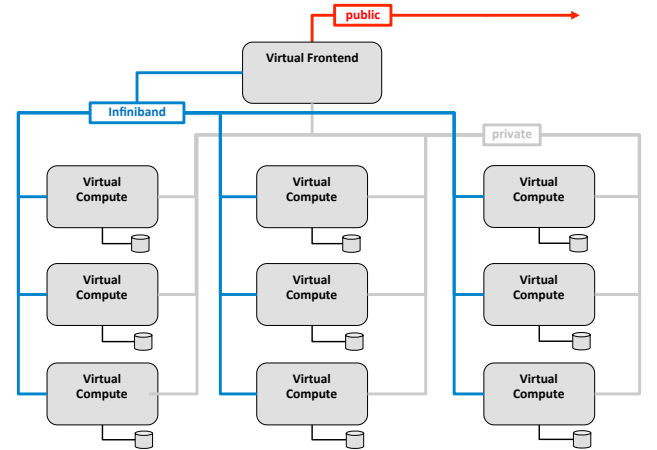
Figure 2: Network topology
