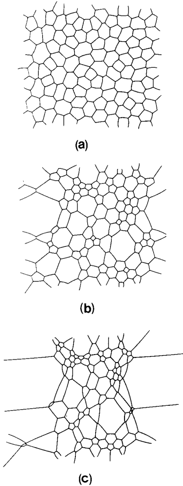
Figure 7. Simulation test of the first-order model, with initial A_{\text{mean}} = 6.75 , C = 0.4 , showing an instability (separation into regions of large and small cells) at \lambda = 1.2 . Results are shown for \lambda = 0.06, 0.36, 1.23 .
