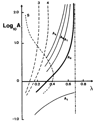
Figure 6. Beyond the point of instability of fivefold cells in figure 5, A_{\text{mean}} (= A_6) should vary as shown here (condition of marginal stability). The resulting variations of A_5 , A_7 , A_8 , A_9 are also shown. The trajectories labelled 3 and 4 give the loci of instability of three- and four-sided cells (cf figure 5). That labelled S denotes the estimated point of the 'spinodal instability', discussed in the text, as a function of A_{\text{mean}} and \lambda .
