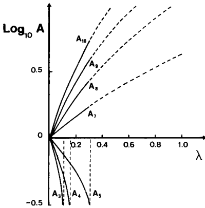
Figure 5. Logarithm of cell area A_n , as obtained by solving (9) for A , setting A_{\text{mean}} (= A_6) = 1.0 and the cut-off parameter C = 1.0 . Three-, four- and five-sided cells become unstable at the points indicated, for this value of A_{\text{mean}} .
