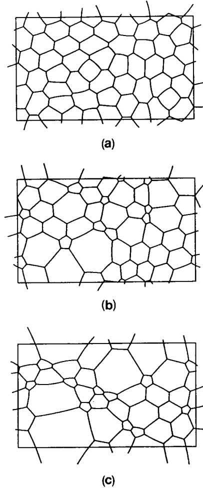
Figure 8. Simulation test of the second-order model, with \kappa_2 = 1 , A_{\text{mean}} = 2.6 , and C = 1.0 . Results are shown for \lambda = 0.01, 0.49, 0.50 .
