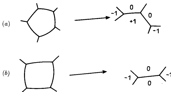
Figure 13. (a) Topological process: disappearance of a five-sided cell. The numbers indicate the change of number of sides of each neighbouring cell. (b) Disappearance of a four-sided cell (created by the process shown in (a)).
