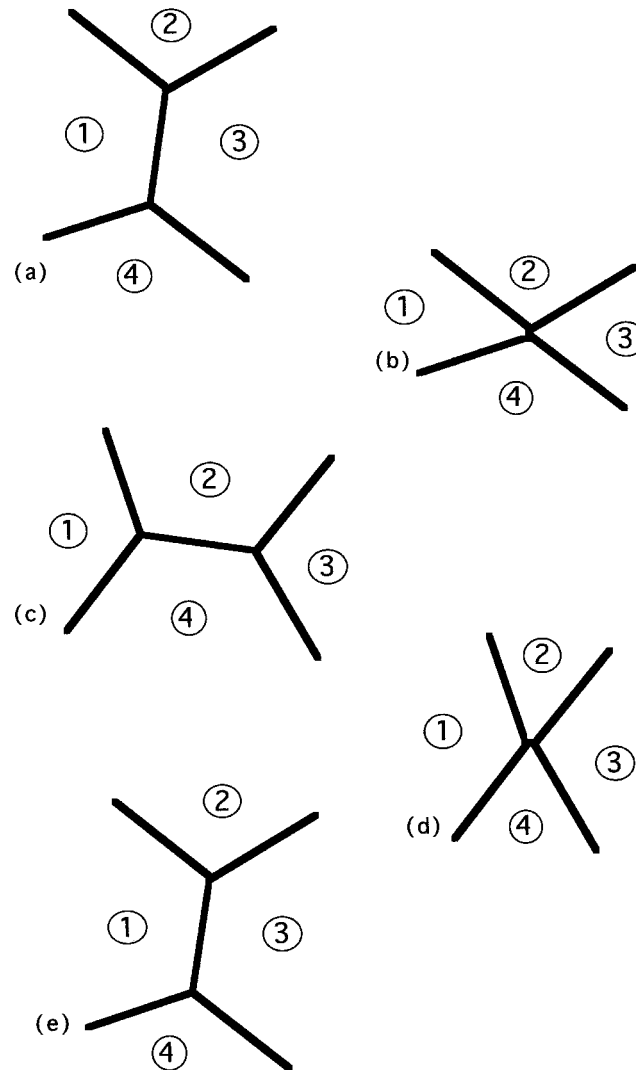
Figure 1. Side swapping (T1 processes). (a) The initial configuration has two threefold vertices. (b) When the side length decreases to zero, an unstable fourfold vertex appears and eventually decays into a new local energy minimum. (c) Cells 1 and 3 lose one side. The reverse T1 (c)–(e) occurs via a different unstable fourfold vertex (d).
