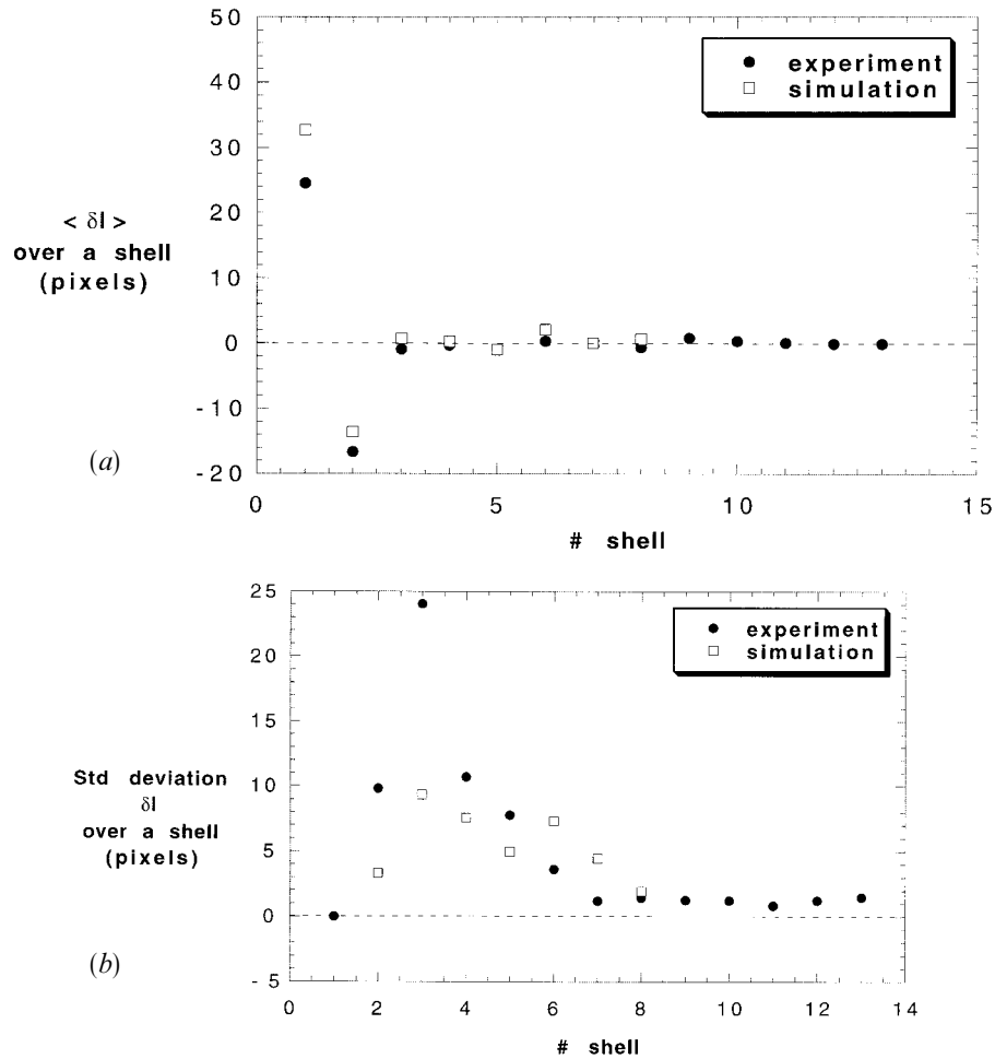
Figure 6. (a) The average side length variation and (b) its standard deviation are measured for each cell wall of a foam before and after a natural T1 process, in an experiment (●) and in a simulation (□). To show the range over which the perturbation due to the T1 extends, the variation for each wall is then averaged over each wall shell , defined as follows. Shell 1 is the disappearing or created wall. Walls of shell 2 touch shell 1, walls of shell 3 touch shell 2, and so on. The shells are therefore roughly circular and centred on the disappearing wall. The last affected shell is shell 6 or 7, that is walls which are separated from the T1 by roughly three cell diameters.
