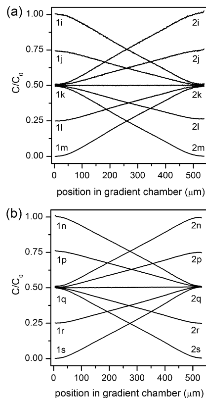
Figure 8. Gradient profiles at l = 100 \mu\text{m} along the dashed line shown in Figure 4 for device 3-20-60 with (a) pressure-driven and (b) electrokinetic flow. The gradients had a constant offset ( C/C_0 = 0.5 ) and varying slopes. Inputs from inlets 1 and 2 correspond to positions in the gradient chamber at 0 and 540 \mu\text{m} , respectively.
