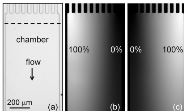
Figure 4. (a) Transmitted-light image of the gradient chamber for device 3-20-60. The chamber is 540 \mu\text{m} wide. Fluorescence images of the gradient for pressure-driven flow with (b) 100% sample at inlet 1 and 0% sample at inlet 2 and (c) 0% sample at inlet 1 and 100% sample at inlet 2. The inflow to the gradient chamber is in 12.5% increments from 100 to 0% in (b) and 0 to 100% in (c). The dashed line shows the position of the profiles in Figures 5, 6, and 8. The scale is the same in all images.
