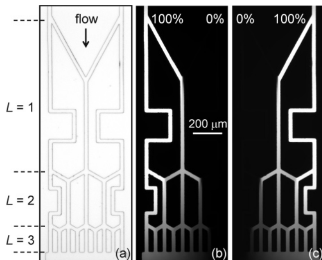
Figure 3. (a) Transmitted-light image of the gradient-forming region for device 3-20-60 with three levels, 20- \mu\text{m} -wide channels, and 9 output channels with 60- \mu\text{m} center-to-center spacing. Fluorescence images of the gradient for pressure-driven flow with (b) 100% sample at inlet 1 and 0% sample at inlet 2 and (c) 0% sample at inlet 1 and 100% sample at inlet 2. The output channels have concentration steps of 12.5% from 100 to 0% in (b) and 0 to 100% in (c). The scale is the same in all images.
