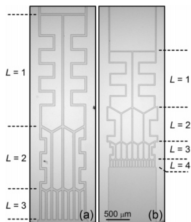
Figure 6. Transmitted-light images of the gradient-forming region for (a) device 3-40-120 and (b) device 4-20-60. Device 3-40-120 has three levels, 40- \mu\text{m} -wide channels, and 9 output channels with 120- \mu\text{m} center-to-center spacing, and device 4-20-60 has four levels, 20- \mu\text{m} -wide channels, and 17 output channels with 60- \mu\text{m} center-to-center spacing. The scale is the same in both images.
