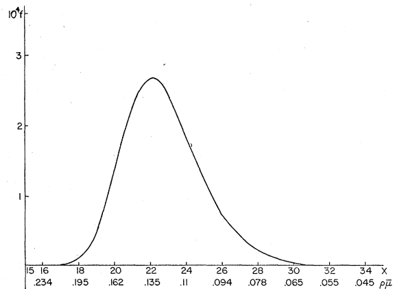
FIG. 9. The density of instantons, 10^4 f(x) , in the dilute QCD phase. f(x)dx represents the fraction of space-time occupied by instantons of scale size between \rho and \rho + d\rho , where \rho\bar{\mu} = \exp(-x/11) , and f(x) = (0.1\pi^2/11)x^6 \times \exp[-x(1 + \alpha e^{-4x/11})] ( \alpha \approx 320 ).
