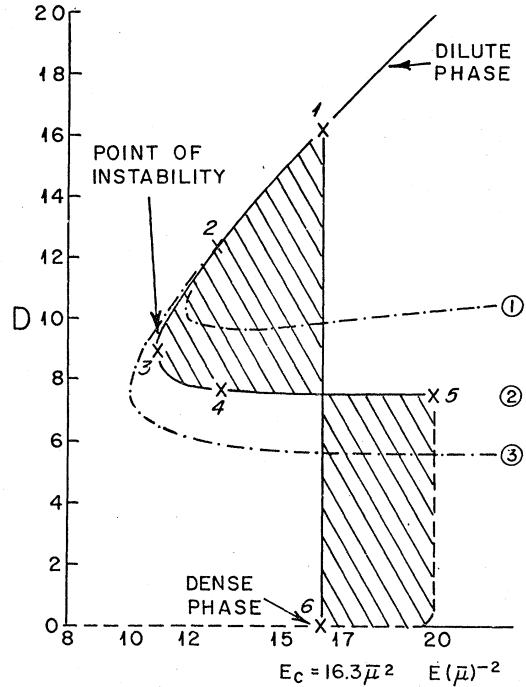
FIG. 6. The equation of state, D(E) , of the QCD vacuum in the presence of an external field E , in units of \bar{\mu}^2 ( \bar{\mu} = renormalization scale parameter), with instanton interactions taken into account. The solid curve holds for a cavity size R\bar{\mu} = 0.42 , whereas the dash-dotted curves (labeled 1 and 3) refer to R\bar{\mu} = 0.34 and 0.55, respectively.
