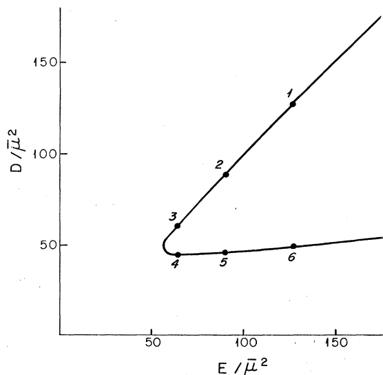
FIG. 8. The D vs E curve for the dimensional renormalization scheme. Values of \mu , etc., at the labeled points are tabulated in Table IV.
