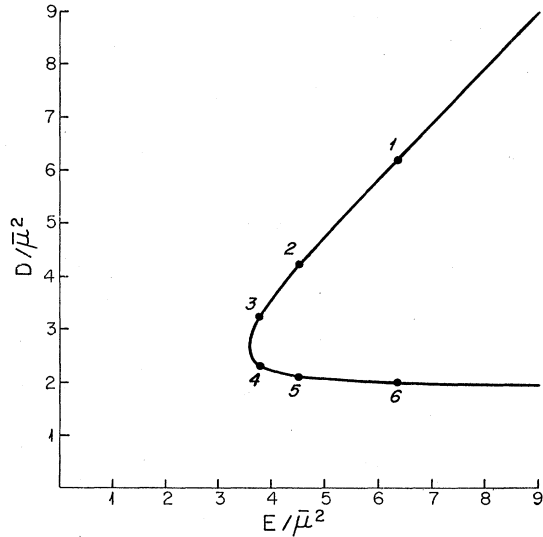
FIG. 7. The D vs E curve for the Pauli-Villars renormalization scheme. Values of \mu , etc., at the labeled points are tabulated in Table III.
