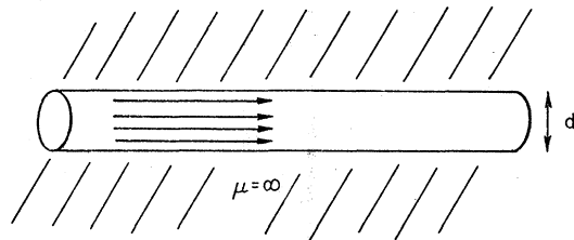
FIG. 10. A flux tube (of diameter d ) for very-well-separated heavy quarks.
