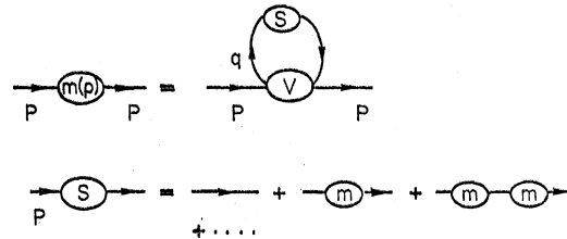
FIG. 11. The Hartree-Fock equations (dilute-gas approximation) to the quark propagator. The instanton-induced determinantal interaction, represented by V , generates, for moderate instanton densities, a dynamical quark mass m(p) .
