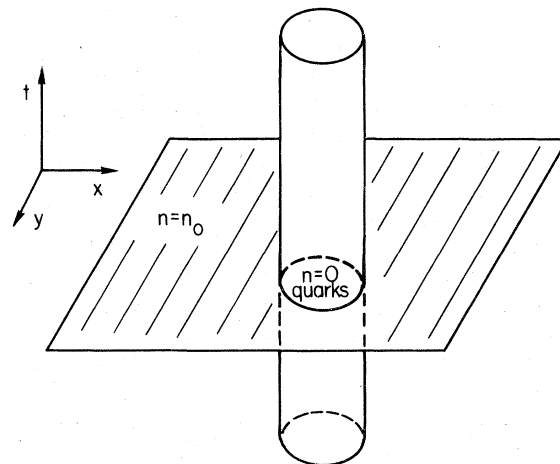
FIG. 2. A static bubble or bag in the QCD vacuum. The cylindrical region corresponds to a region of space, whose time histories have no instanton or meron pair tunneling events.
