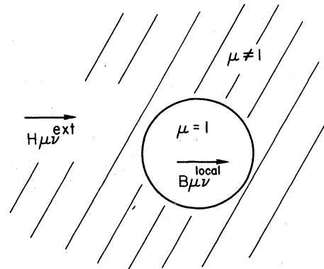
FIG. 1. A spherical cavity with \mu=1 in a paramagnetic medium with \mu \neq 1 .
