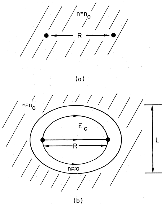
FIG. 4. (a) Quark in a uniform sea of instantons and meron pairs. (b) Quarks in a bubble or bag in the shape of a flux tube.
