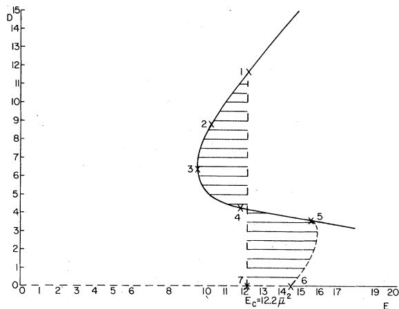
FIG. 5. The equation of state, D(E) , of the QCD vacuum in the presence of an external field E , in units of \bar{\mu}^2 ( \bar{\mu} = renormalization scale parameter), without instanton interactions taken into account.
