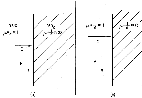
FIG. 3. (a) The boundary conditions at the surface of a perfect paramagnet (QCD vacuum). (b) The boundary conditions at the surface of a perfect diamagnet (superconductor or Higgs vacuum).
