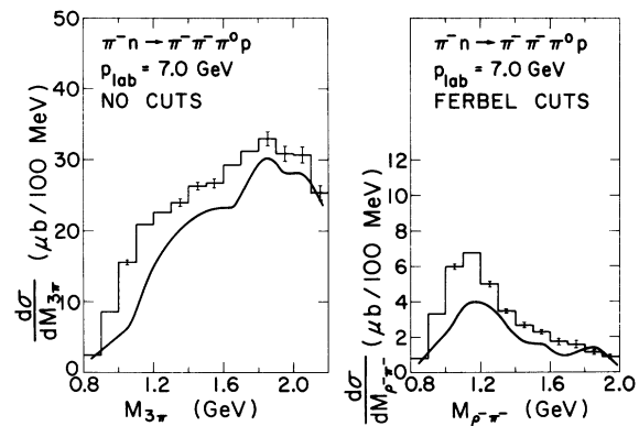
FIG. 20. (a) The 3\pi mass in \pi^-n \rightarrow \pi^- \pi^- \pi^0 p . Curve is drawn by hand through data from Ref. 21; histogram is prediction of our model. (b) The \rho^-\pi^- mass spectrum in \pi^-n \rightarrow \pi^- \pi^- \pi^0 p after Ferbel cuts ( |t_{\rho-\pi^-}| < 0.5 \text{ GeV}^2 , M_{\rho\pi^-} > 1.5 \text{ GeV} ) were made. The curve is drawn by hand through data from Ref. 22; histogram is the prediction of our model.
