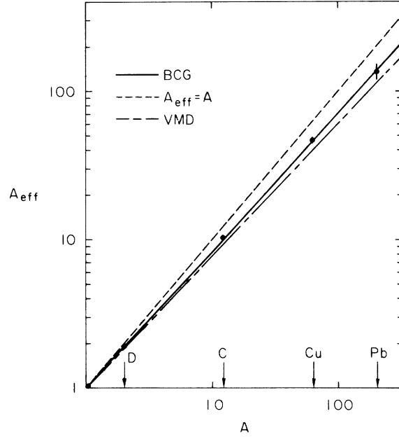
FIG. 6. Shadowing in 14.4–18.3 GeV on-shell nuclear photoabsorption. A_{\text{eff}} = \sigma(\gamma A)/\sigma(\gamma N) for a nucleus containing A nucleons. "No shadowing" would predict A_{\text{eff}} \sim A (the upper curve) while the VMD model with \sigma(\rho N) = 26 mb and a ratio of 20% for the real part of the \gamma \rightarrow \rho amplitude to its imaginary part yields the lower curve ( \gamma_\rho^2/4\pi = 0.65 ). The curve labeled BCG is given by 0.22A + 0.78A^{0.89} (see text), corresponding to the 22% pointlike portion expected on the basis of the model of the text.
