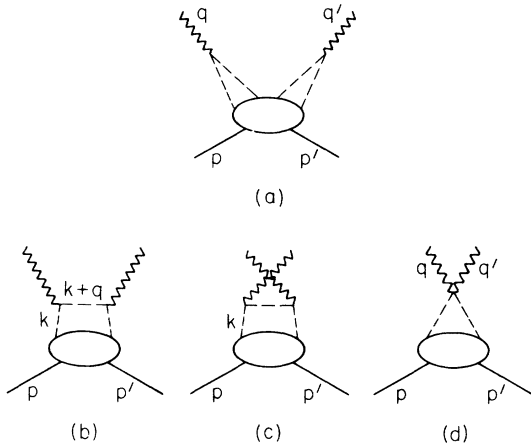
FIG. 1. The covariant diagrams contributing to the Compton amplitude. In the text these are referred to as (a) six-point or T^{(6)} , (b) and (c) four-point or T^{(4)} , (d) seagull. (d) is separable from (b) and (c) only for spin-0 partons (see text and Ref. 1).
