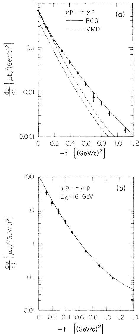
FIG. 4. Compton scattering at 16.6 GeV/c [data from R. L. Anderson et al. , Phys. Rev. Letters 25, 1218 (1970); A. M. Boyarski et al. , ibid. 26, 1600 (1971)]. The lower of the curves labeled VMD is the result of taking the vector-meson photoproduction data of Ref. 8 and using \gamma_\rho^2/4\pi = 0.65 (see text). [This of course is the Orsay value and is also that which works well in predicting \gamma V from VV data; see Fig. 4(b) where we show a sample comparison between this latter VMD prediction and the \gamma V data.] Renormalizing this curve so as to agree at small t yields the upper VMD curve (corresponding to \gamma_\rho^2/4\pi = 0.35 ). The curve labeled BCG is that described in Ref. 14.
