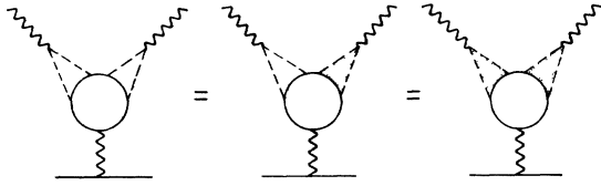
FIG. 3. The single-Regge limit of the T^{(6)} diagram appropriate in the Regge region of Compton scattering. Also shown schematically is the VMD hypothesis for this diagram, which relates (a) \gamma\gamma to (b) \gamma V , and to (c) VV . VMD applies only to the T^{(6)} diagrams.
