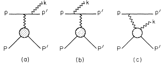
FIG. 5. The Feynman diagrams contributing to the process e p \rightarrow e p \gamma to lowest order in e . (a) and (b) are the Bethe-Heitler processes, and (c) is the Compton contribution. Note that when e^+ \rightarrow e^- , diagram (c) changes sign whereas (a) and (b) are unchanged.
