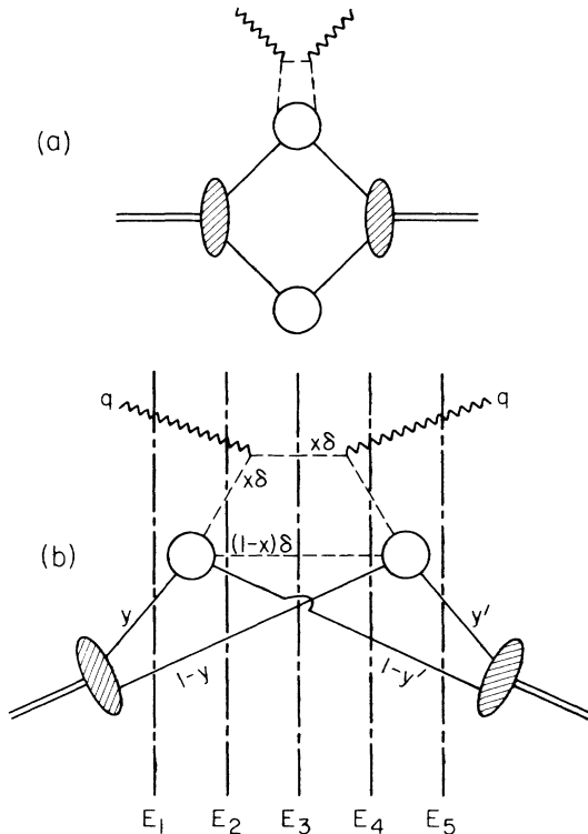
FIG. 7. Nuclear shadowing of the four-point contribution to Compton scattering. (a) The deuteron becomes two nucleons and the Compton scattering takes place on a parton of one nucleon, the parton being reabsorbed by the same nucleon. The nucleons then recombine to form the deuteron. (b) The process that might shadow the pointlike one of (a). In this case the parton which is involved in the Compton scattering is reabsorbed by a different nucleon than that from which it was emitted. In addition a second parton travels between the two nucleons.
