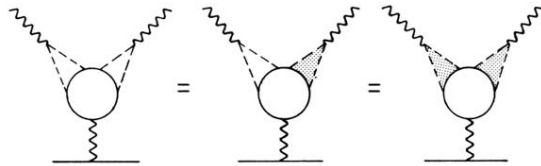
FIG. 3. The single-Regge limit of the T^{(6)} diagram appropriate in the Regge region of Compton scattering. Also shown schematically is the VMD hypothesis for this diagram, which relates (a) \gamma\gamma to (b) \gamma V , and to (c) VV . VMD applies only to the T^{(6)} diagrams.
