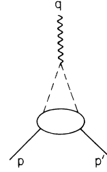
FIG. 2. The elastic form factor.
