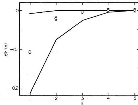
FIG. 7. As in Fig. 6, but for 4/g_0^2=2 . For this lattice 4/g_0^{*2}=1.85 . The lower curve is the screened Coulomb potential in the color-singlet channel; the upper curve is the color-averaged screened Coulomb potential.
