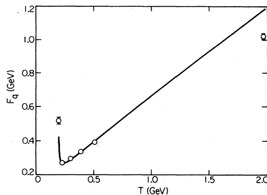
FIG. 4. Quark free energy vs temperature. The points and the curve result from simple transformations of Fig. 3.
