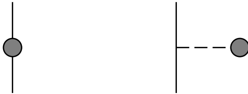
Figure 2.1: The Feynman graphs which give the dominant nucleon matrix elements of the Noether currents in the low-energy effective theory. Solid lines represent nucleons, and dashed lines represent pions.
