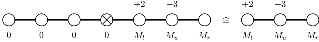
Figure 4: Reduction of the distinguished Dynkin diagram of SU(4|2,2) to SU(2,2) . Above the diagrams we have indicated the Dynkin labels of the spin representation and below the excitation numbers of each simple root.
