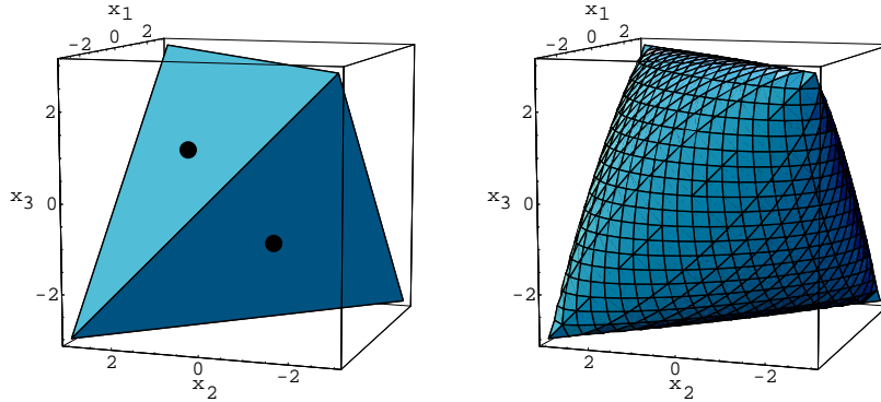
Figure 18: The fundamental domain (left) for constant gauge fields on S^3 , with respect to the framing \tilde{e}_\mu^j , in the diagonal representation A_j = x_j \sigma_j (no sum over j ). The dots on the faces indicate the sphalerons. On the right we show the Gribov horizon, which encloses the fundamental domain, coinciding with it at the singular boundary points along the edges of the tetrahedron.
