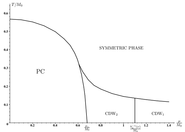
FIG. 9. The (\mu, T) phase portrait at fixed \nu , where \nu_\alpha < \nu . Here b_0^{-1}(\nu) is the function inverse to b_0(\mu) defined in Fig. 3. PC denotes the homogeneous charged pion condensation phase with M = 0, b = 0, \Delta = M_0 . CDW_2 denotes the inhomogeneous chiral density wave phase with b < 0 . All critical curves do not depend on \nu . Other notations are the same as in the previous figures.
