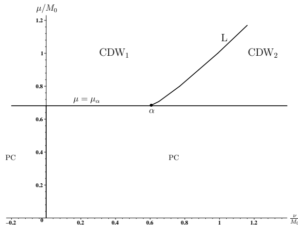
FIG. 7. The (\nu, \mu) phase portrait of the model at T = 0 when a spatial CDW inhomogeneity is taken into account. In the CDW_1 ( CDW_2 ) phase b > 0 ( b < 0 ). The curve L, on which b = 0 , corresponds to the homogeneous chiral symmetry broken phase. The same is true for the interval 0 < \mu < \mu_\alpha of the \mu -axis, where \mu_\alpha = \mu_c \approx 0.68M_0 .
