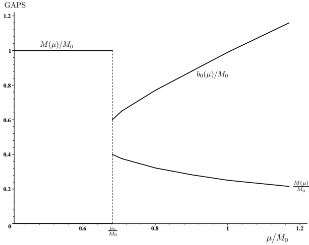
FIG. 3. The CDW amplitude M(\mu) and its wave vector b_0(\mu) as functions of \mu in the case of zero isospin chemical potential. Here \mu_c = \mu_\alpha \approx 0.68M_0 .
