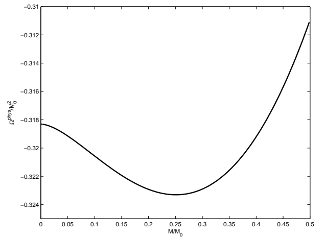
FIG. 6. Section of the plot of \Omega^{\text{phys}} (33) vs M at \mu = M_0 along the axis M passing through the point of minimum.
