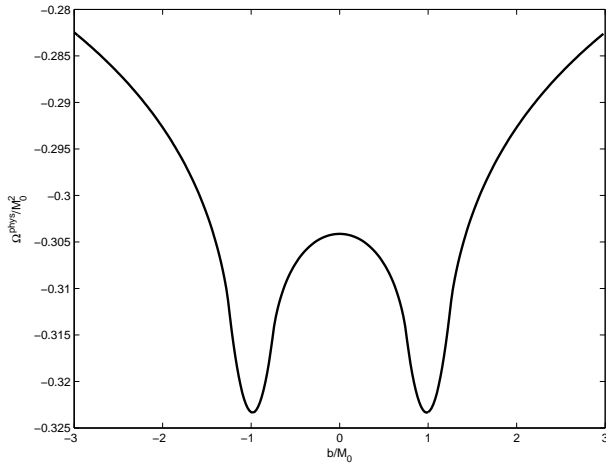
FIG. 5. Section of the plot of \Omega^{\text{phys}} (33) vs b at \mu = M_0 along the axis b passing through the point of minimum.
