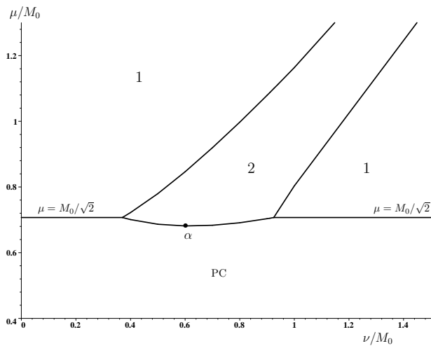
FIG. 1. The (\mu, \nu) phase portrait of the model considered at T = 0 and \nu > 0 in the case of spatially homogeneous condensates. Here \nu = \frac{\mu_I}{2} , and M_0 is the quark mass in the vacuum. Number 1 denotes the symmetric phase with massless quarks, number 2 the normal quark matter phase with massive quarks, and PC denotes the charged pion condensed phase. The point \alpha is the lowest point of the phase 2: \mu_\alpha \approx 0.68M_0 , \nu_\alpha \approx 0.6M_0 .
