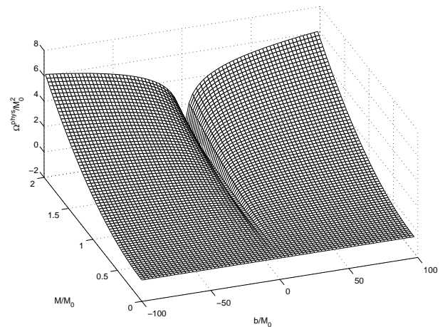
FIG. 2. The plot of \Omega^{\text{phys}} (30) vs M, b at \mu_I = 0, \mu = M_0, \Delta = 0 .
