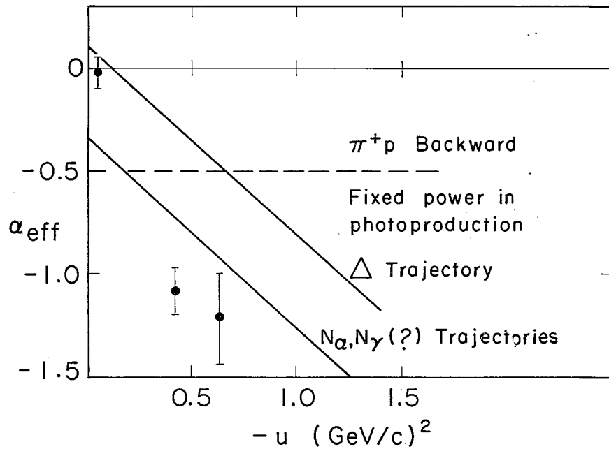
Fig. 18. \pi^+ p \rightarrow p \pi^+ backward scattering (See Appendix)
