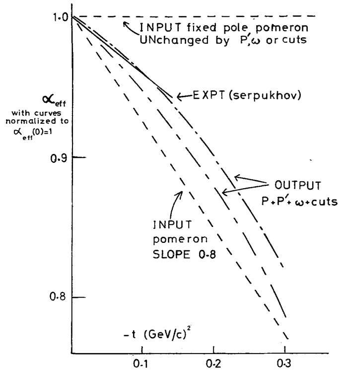
Fig. 30. \alpha_{\text{eff}} for p-p elastic scattering calculated over Serpukhov energies ( p_{\text{lab}} \leq 70 GeV/c). The solid line is the experimental result 43 presented at this conference. Also shown, (---), is a Pomeron of slope 0.8, with the result of adding P' + \omega + \text{cuts} to this (-----). There are two of the latter curves corresponding to two possible P', \omega parameters. Notice the marked curvature of the (-----) lines. This occurs as there is tremendous shrinkage predicted for -t \gtrsim 0.6 (GeV/c) 2 as the pole-cut interference dip moves in, as energy increases.
