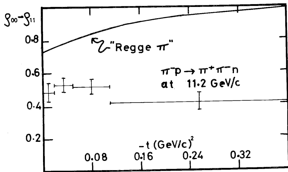
Fig. 42. A comparison of the fit of ref. 74 with the same data as presented in fig. 35. We only show the fit to \rho_{00} - \rho_{11} . The fits to d\sigma/dt and \langle a_0 b_0 \rangle (not shown) are good. Finally this model predicts zero for \rho_{1-1} , \rho_{10} and \langle a_1 b_0 \rangle . (The experimental data is shown in figs. 35 (d), (e) and (f)).
