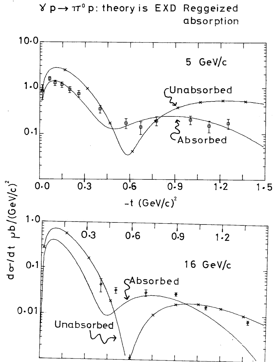
Fig. 33. \pi^0 photoproduction at p_{\text{lab}} of 5 and 16 (GeV/c).
