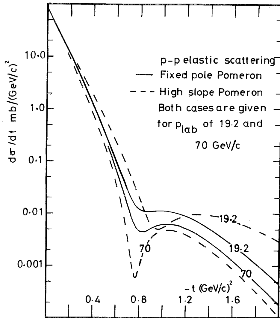
Fig. 29. An indication of the change we may expect in p - p elastic scattering between 19.2 and 70 GeV/c. The parameters used in the calculation came from a best fit to all p - p data. Thus there is poor agreement with experiment at 19.2 GeV/c and so only the relative differences between the curves is of relevance.
