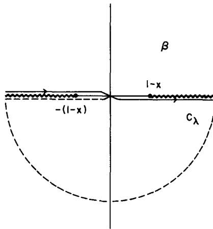
Fig. 1. Integration path C_\lambda .
