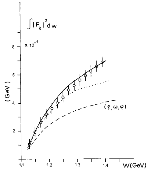
Fig. 2. The duality integral \int |F_K|^2 dW versus W = \sqrt{s} . The solid line is the theoretical curve, the dotted line is without the (\omega_1, \varphi_1) terms and the dashed line is the VDM prediction. The circles give the integrals over the experimental values from ref. [2].
