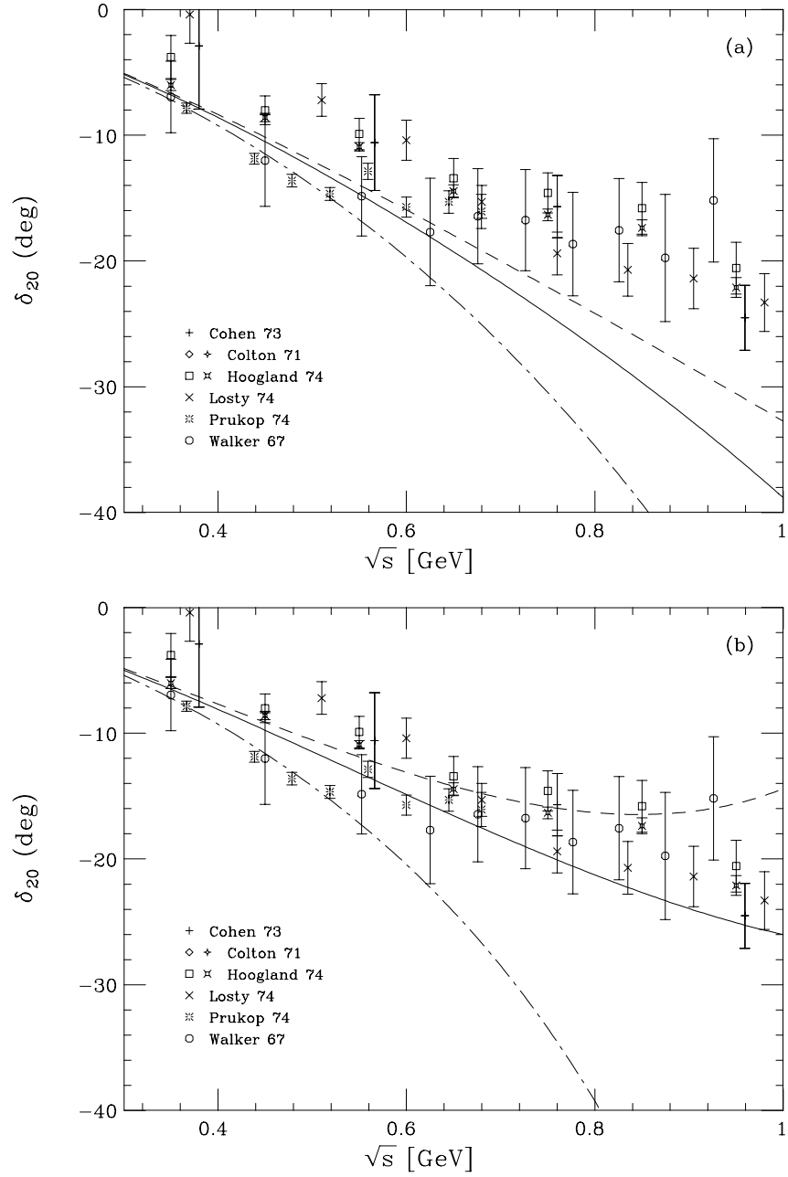
FIG. 3. The I=2 , J=0 \pi\pi phase shift with (a) \rho exchange only; (b) degenerate \sigma and \rho exchanges for the KSUF/Weinberg (dashed), Veneziano (dot-dash), and intermediate g_\rho^2 = 0.45m_\rho^2/2f_\pi^2 (solid) couplings. Some experimental data are also shown.
