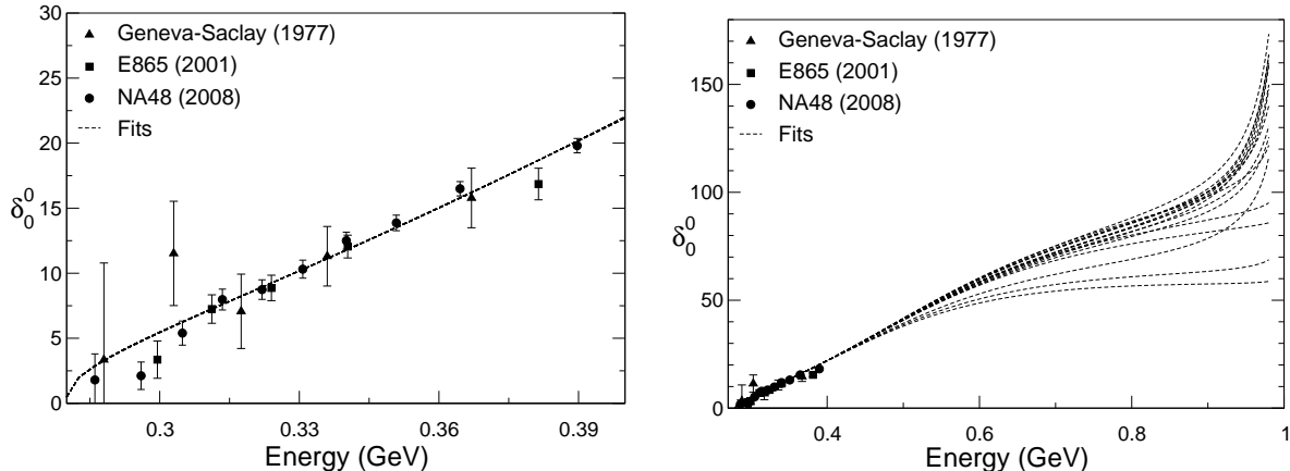
Figure 2: Left: phase shift \delta_0^0 derived from K_{e4} decay, fitted with the 16 parametrizations described in the text. Right: extrapolation of the fits above the experimental range.
