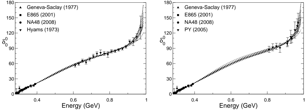
Figure 4: Left: fits of the data in set I ( K_{e4} data [5]-[7] plus the CERN-Munich data [27] below the K\bar{K} threshold). Right: fits of the data in set II ( K_{e4} data plus a selection of data from \pi N \rightarrow \pi\pi N , given in [15]).
