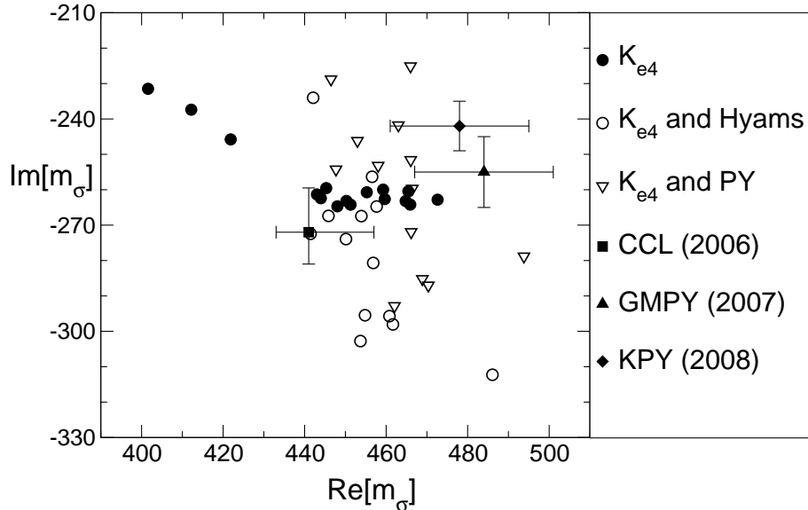
Figure 3: Positions of the \sigma pole obtained by the analytic extrapolation of the parametrizations used for fitting various sets of data, compared with Refs. [4], [8] and [23] (from the last reference we show the value obtained with isospin corrected K_{e4} data).
