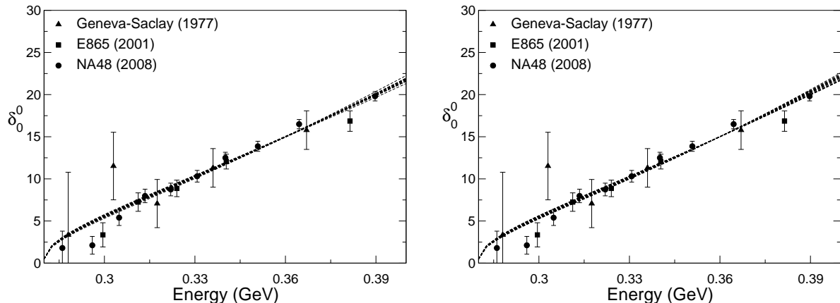
Figure 5: Expanded view of the low energy region from Fig. 4.
