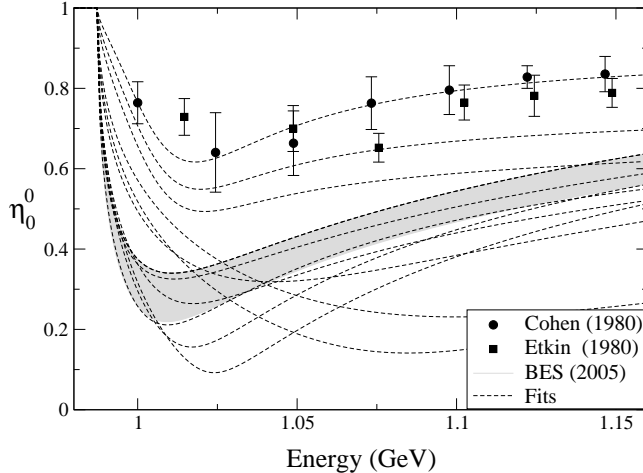
Figure 6: Elasticity \eta_0^0 obtained with the 13 parametrizations of the data in set I (cf. Table 2), compared with the experimental data from [17]-[18].
