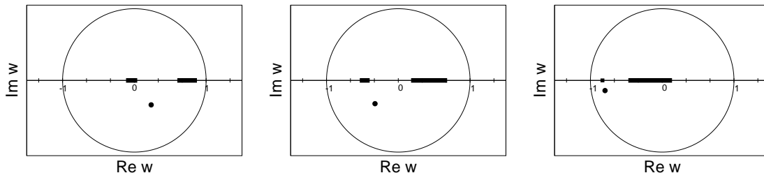
Figure 1: The disk |w| < 1 in the complex plane w = w(s, \alpha) defined in (7), for \alpha = 0.36 (left), \alpha = 1 (center) and \alpha = 4 (right). The thick segments indicate the regions where experimental data are available from K_{e4} decay [5]-[7] and the process \pi N \rightarrow \pi\pi N (cf. the compilation of data made in [15]), respectively; the circle shows the \sigma pole on the second Riemann sheet from [4].
