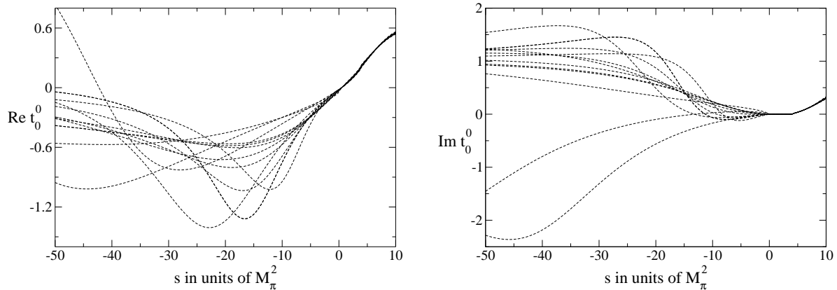
Figure 7: \text{Re } t_0^0(s) (left) and \text{Im } t_0^0(s) (right) obtained by the extrapolation of the 13 parametrizations of the data in set I.
