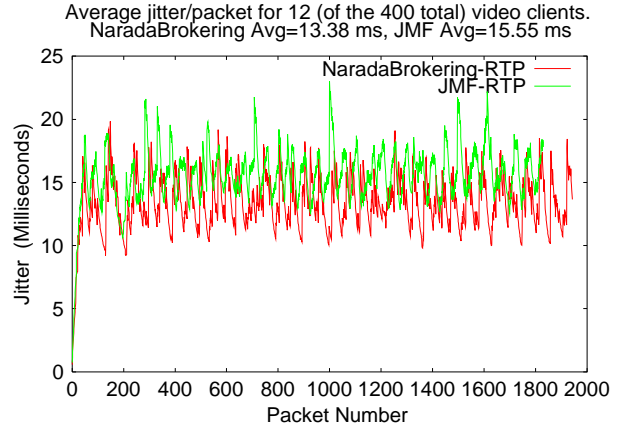
Figure 4. Jitter for 400 video clients
