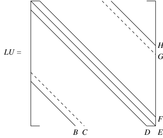
Figure 3: The form of the LU product matrix.
