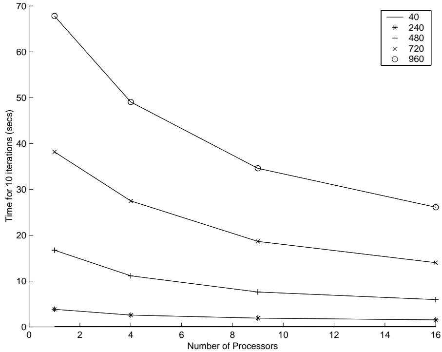
Figure 7: The wavefront method execution times
