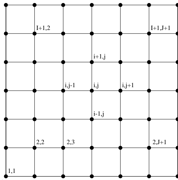
Figure 1: The finite difference stencil
