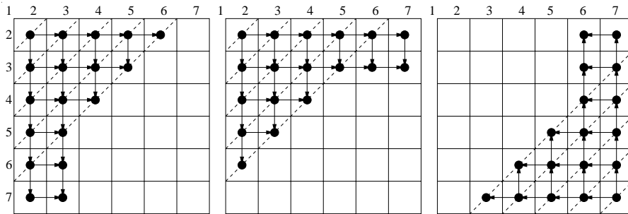
Figure 4: Step 1. Factorisation, 2. Forward Elimination, 3. Backward Substitution
