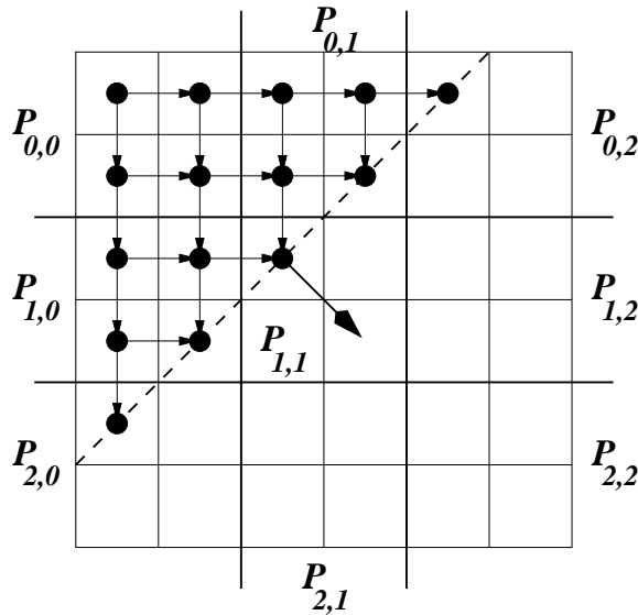
Figure 5: Block checkerboard partition
