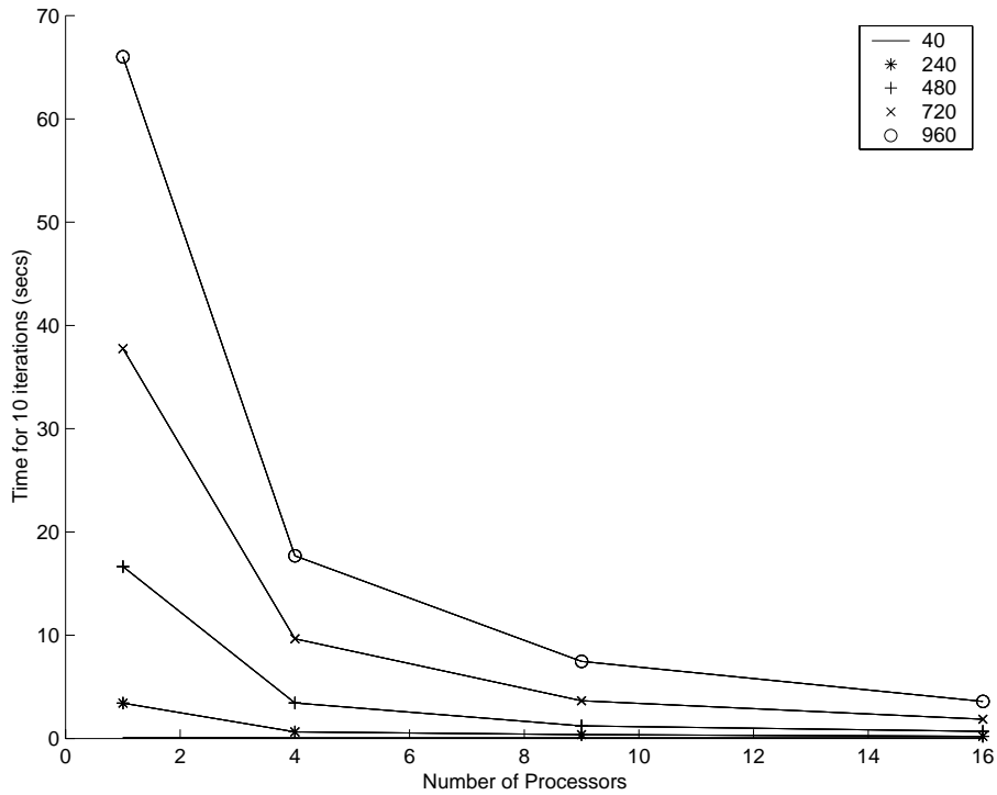
Figure 8: The red-black method execution times
