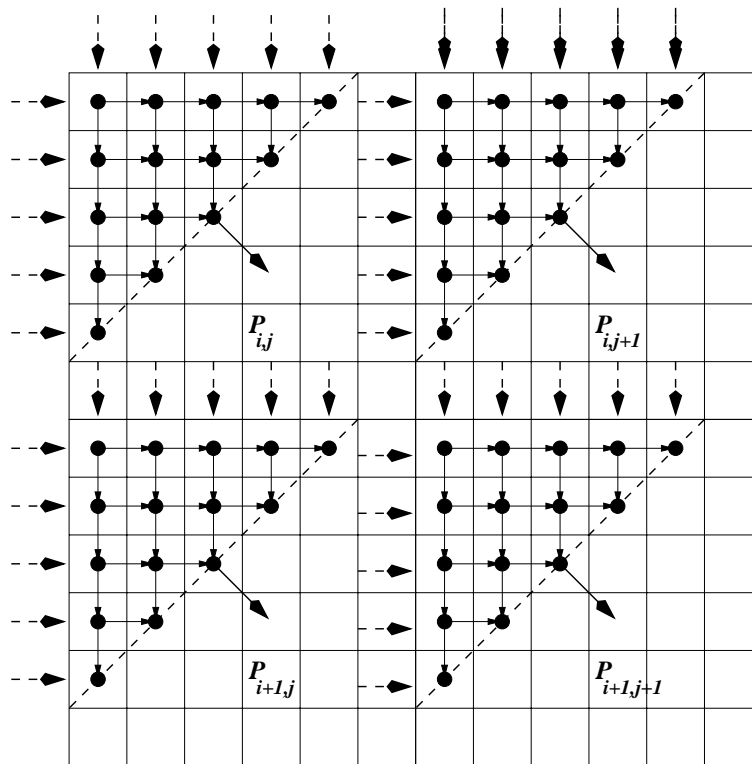
Figure 6: Communications involved in factorisation and forward sweep.
