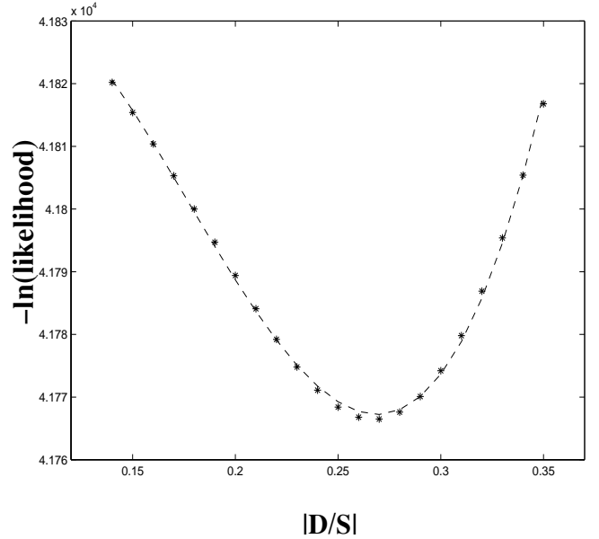
FIG. 8: The projection of the -\ln(\text{likelihood}) as a function of |D/S| . The distribution was fitted to a second order polynomial function, with the minimum at |D/S| = 0.269 \pm 0.009 .
