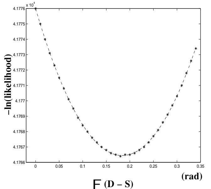
FIG. 9: The projection of the -\ln(\text{likelihood}) as a function of \phi(D-S) . The distribution was fitted to a second order polynomial function, with the minimum at \phi(D-S) = 0.184 \pm 0.042 rad, or 10.54^\circ \pm 2.4^\circ .
