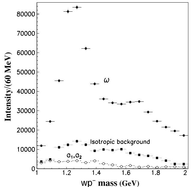
FIG. 4: Acceptance-corrected intensities from various contributions: Filled circles: waves with an \omega in the final state, Squares: “isotropic wave, Open circles: waves with either an a_1 or an a_2 in the final state.
