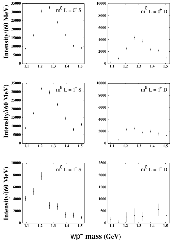
FIG. 6: Acceptance-corrected intensities for the J^{pc} = 1^{+-} m^\epsilon L partial waves. Only the positive reflectivity waves are used in the measurement of D/S . Notice the different ordinate scale for the weaker negative reflectivity signals.
