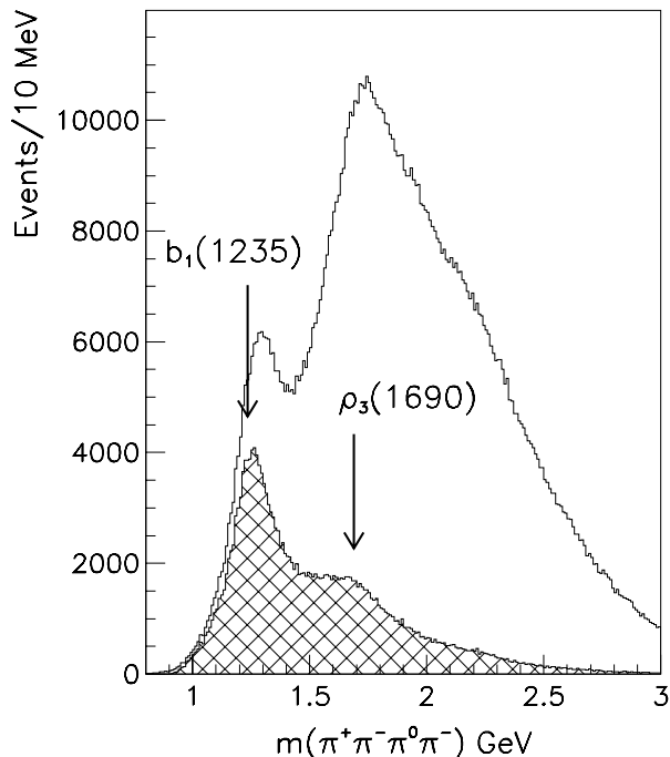
FIG. 2: Invariant mass spectrum for \pi^+\pi^-\pi^0\pi^- and \omega\pi^- combinations. The hatched regions correspond to an \omega mass cut.
