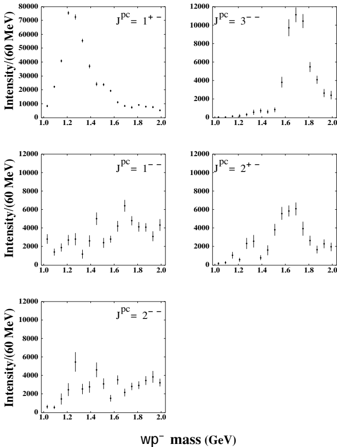
FIG. 5: Acceptance-corrected intensities from the results of a PWA fit. The list of \omega waves included in this fit is shown in Table I. Individual contributions for different J^{pc} are shown. Each J^{pc} is the sum of the allowed m^\epsilon L included in the fit.
