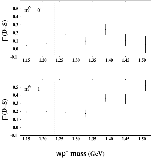
FIG. 7: Phase differences between the 1^{+-}m^e D and S waves with positive reflectivity, m^e = 0^+ ( 1^+ ) in the top (bottom) plot. The dashed lines are drawn at the mass of the b_1 to guide the eyes.
