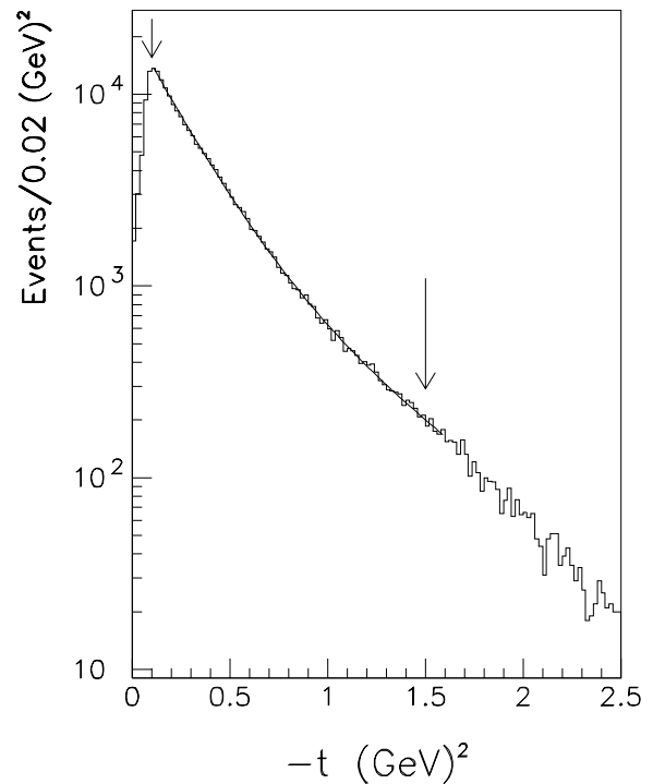
FIG. 3: The negative of the four-momentum transfer squared, -t distribution for the \omega\pi^-p final state. The distribution is fitted to the sum of two exponential functions. The fit results yield two slopes, P2 = 4.5 \pm 0.052 \text{ (GeV}^2\text{)}^{-1} and P4 = 1.7 \pm 0.070 \text{ (GeV}^2\text{)}^{-1} . The arrows indicate the region chosen in the PWA: (0.1 < -t < 1.5 \text{ (GeV}^2\text{)}) .
