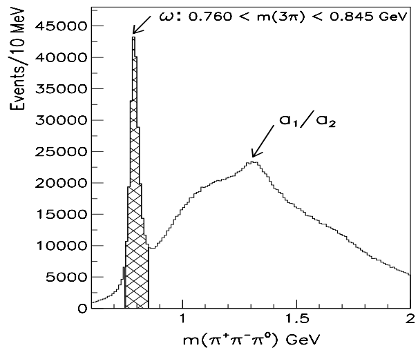
FIG. 1: Invariant mass spectrum for \pi^+\pi^-\pi^0
