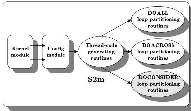
Figure 4: The structure of s2m .
