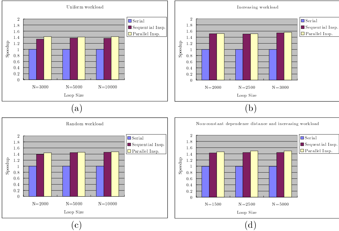
Figure 20: Results of runtime parallelization.
