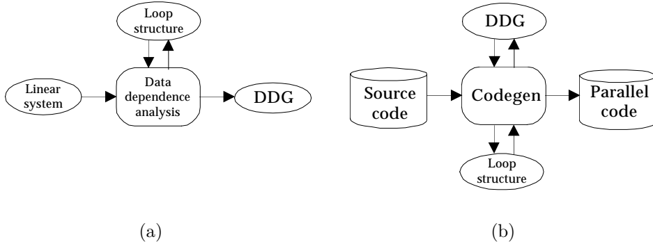
Figure 3: An overview of the analysis and codegen phases.
