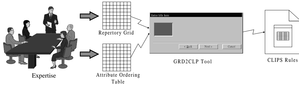
Figure 9: The process of generating a knowledge base
