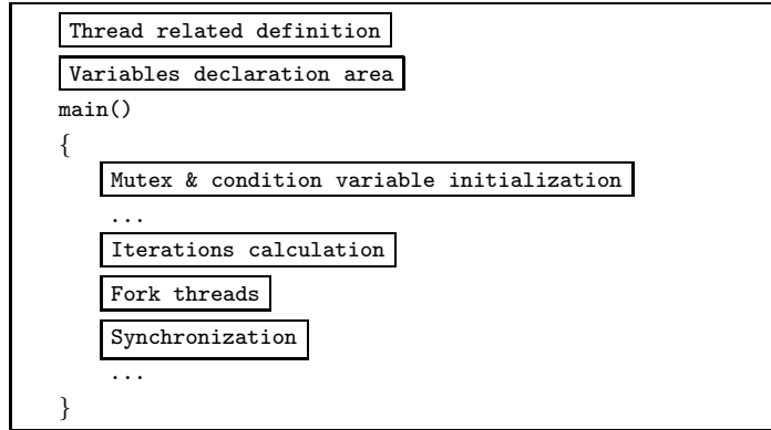
Figure 6: Main program of the general output produced by s2m.
