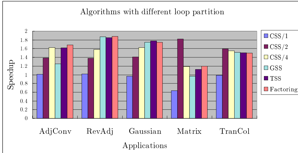
Figure 17: Result of different loop-partitioning algorithms.
