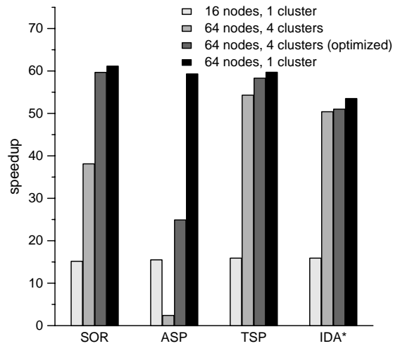
Figure 7: Speedups of four Java applications on a single cluster of 16 nodes, 4 WAN-connected clusters of 16 nodes (original and optimized program), and a single cluster of 64 nodes.
