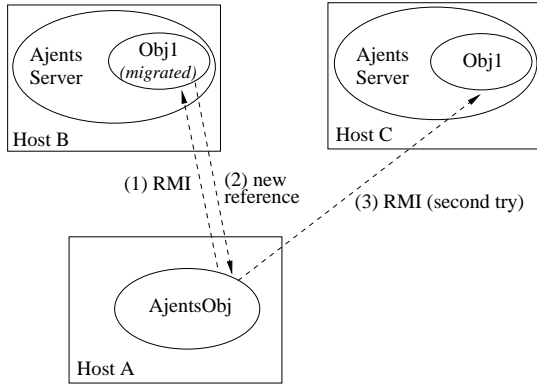
Figure 3: Example of a remote method invocation after a third party migration.
