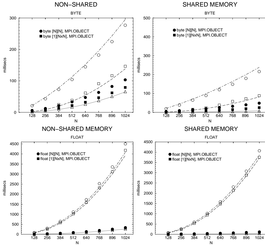
Figure 7: Timings allowing two-dimensional array proxies in the object stream (solid points).
