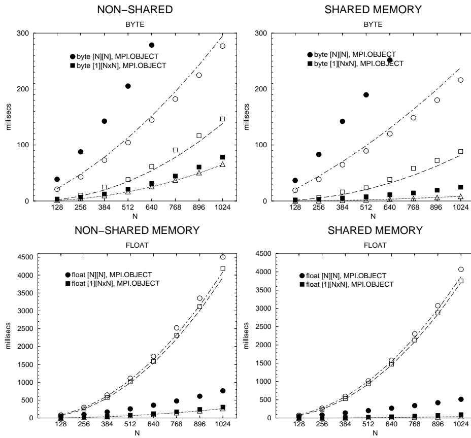
Figure 6: Pingpong timings with primitive array data sent separately (solid points), compared with results in Figure 3.
