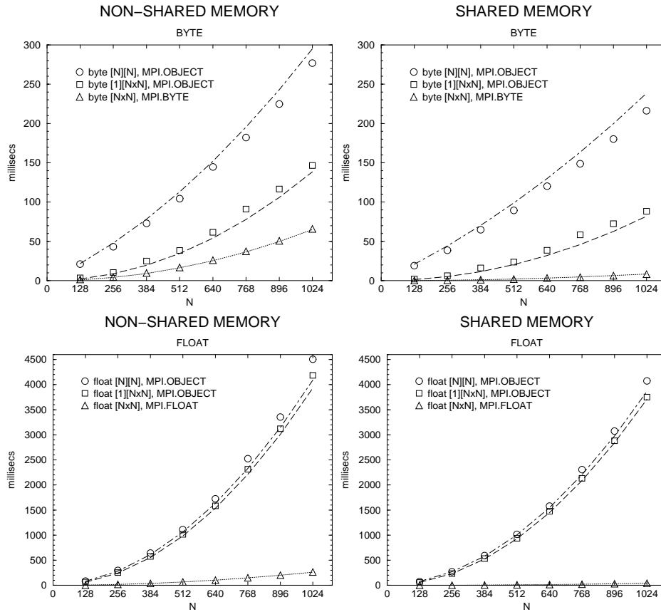
Figure 3: Communication times from Pingpong benchmark in non-shared-memory and shared-memory cases, compared with model defined by Equations 1 to 3 and Table 1.
