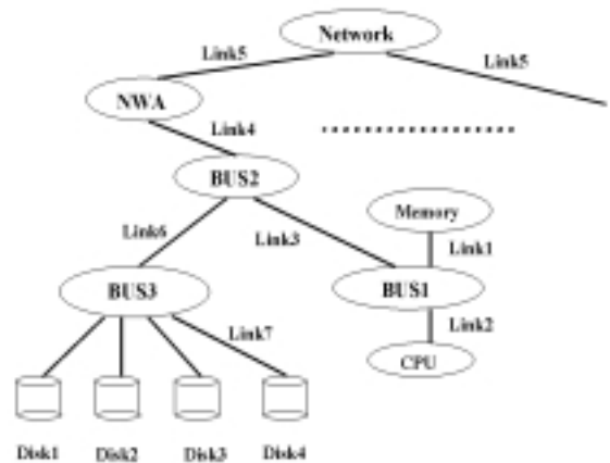
Fig.3: Typical SP2 configuration used in fig. 4 showing the nodeset and linkset components
