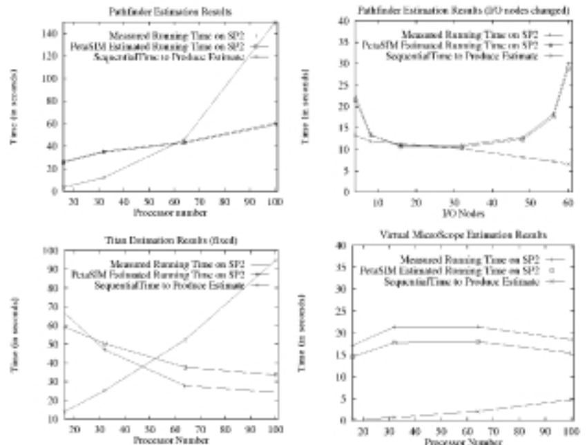
Fig.4: Measured Execution Time compared to the estimated execution time from PetaSIM for four examples. We also show the sequential execution time needed to produce the estimate.
