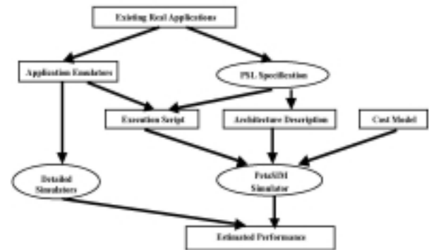
Fig.1: The Performance Prediction Process
