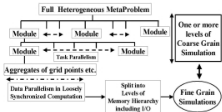
Fig. 5: Support for coarse grain modules in PetaSIM
