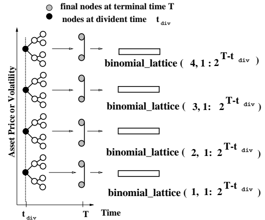
Figure 3: Binomial lattice expressed as a two-dimensional array
