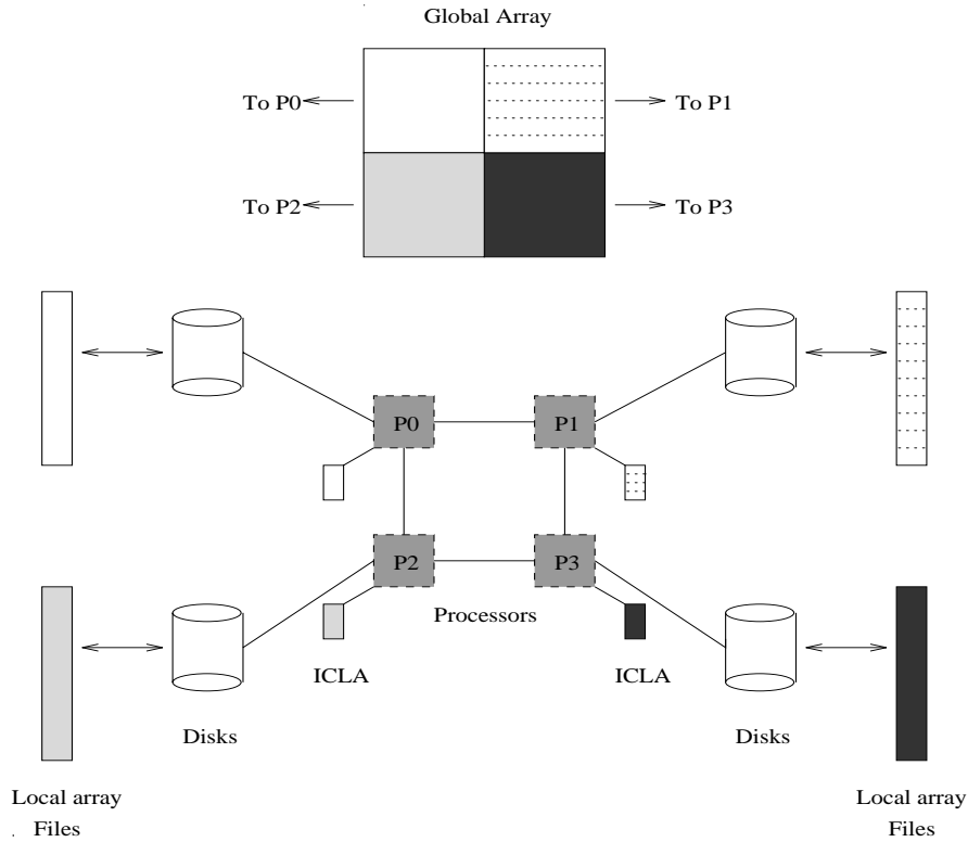
Figure 2: Model for Computation and I/O
