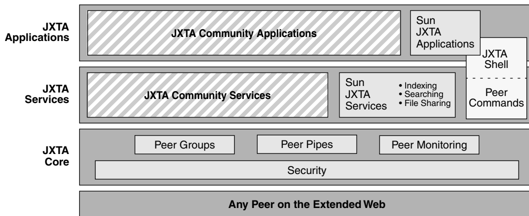
Figure 1: P2P Software Architecture
