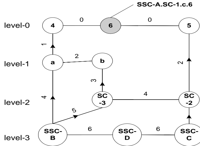
Figure 4.3: The connectivity graph at node 6.
