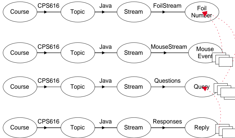
Figure 5.1: The stream context graph for 4 related streams.
