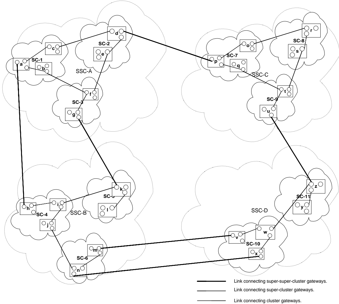
Figure 3.3: Gatekeepers and the organization of the system
