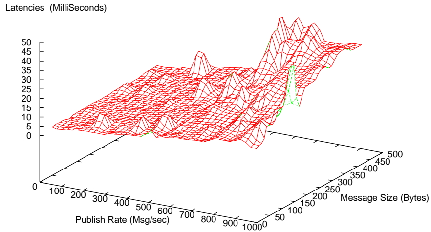
Subscriber 2 server hops from publisher - Matching 10%
