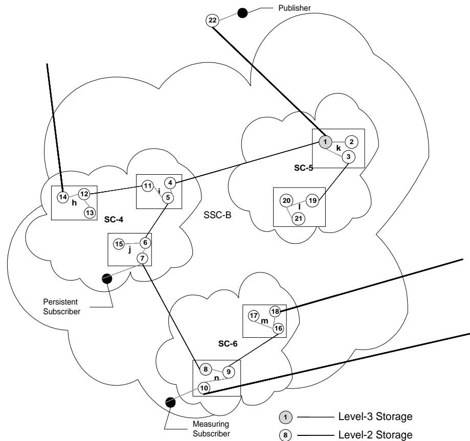
Figure 7.1: Testing Topology
