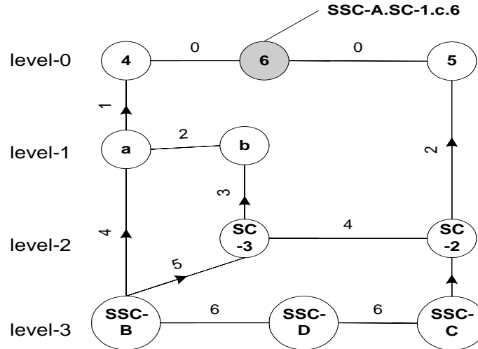
Figure 6.4: The connectivity graph at node 6 and the detection of partitions.
