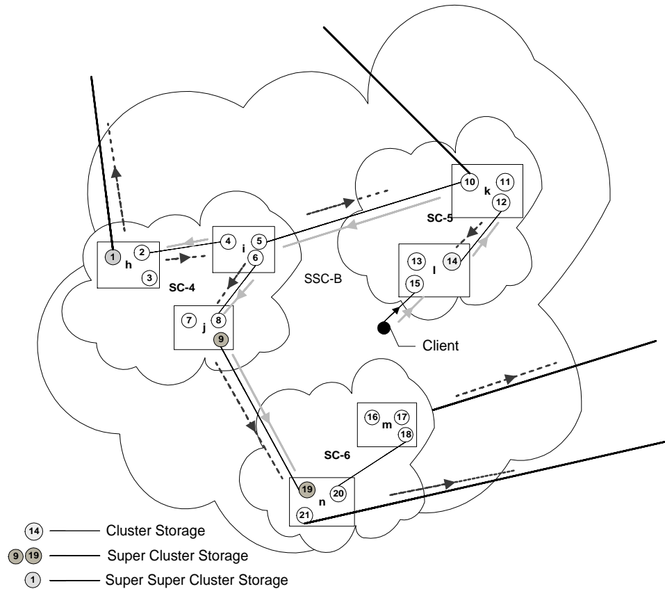
Figure 6.8: The propagation of events in the system
