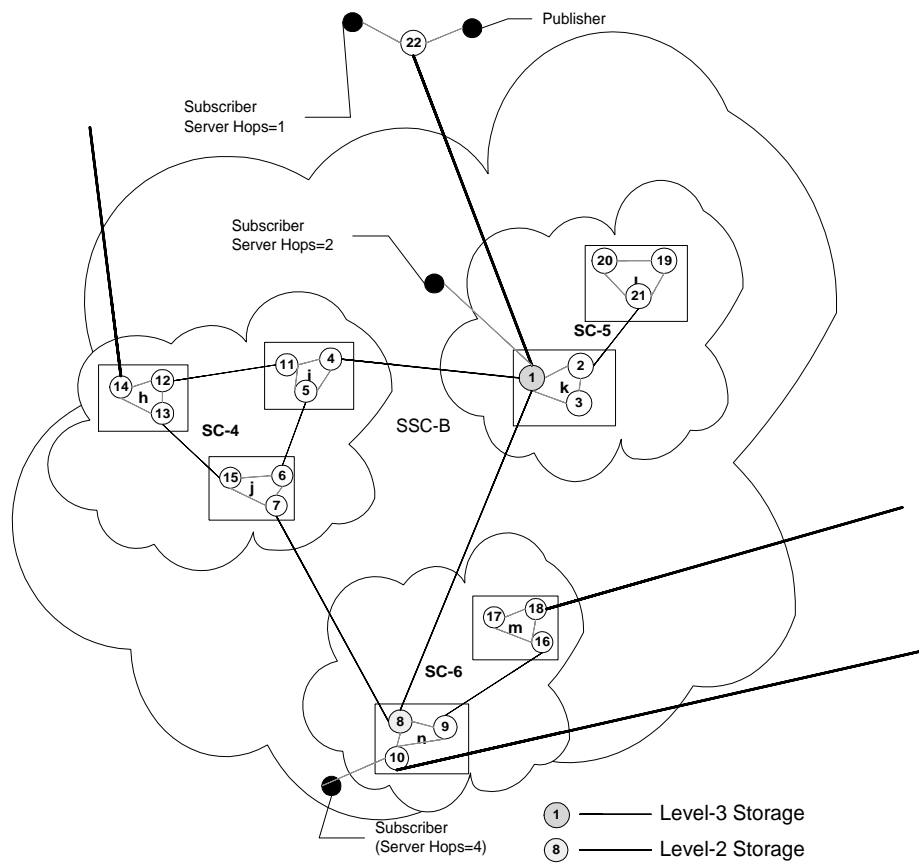
Figure 7.9: Testing Topology - Latencies versus server hops
