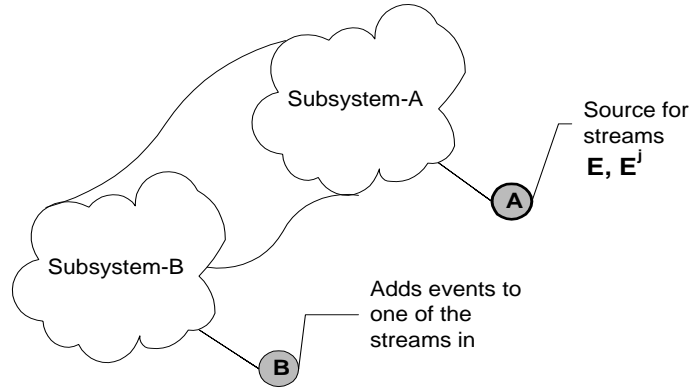
Figure 5.3: Resolving dependencies.
