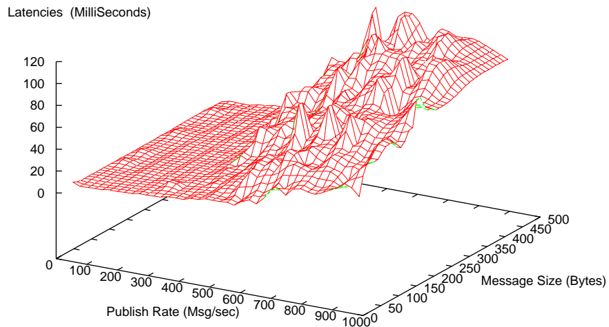
Subscriber 2 server hops from publisher - Matching 50%
