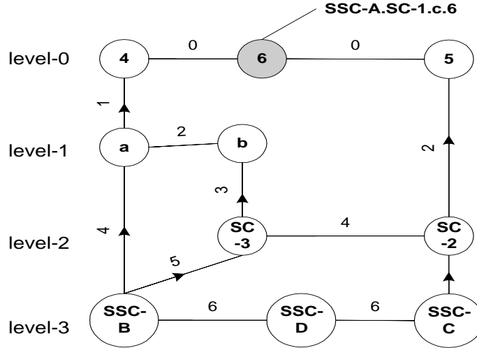
Figure 4.7: The connectivity graph at node 6.
