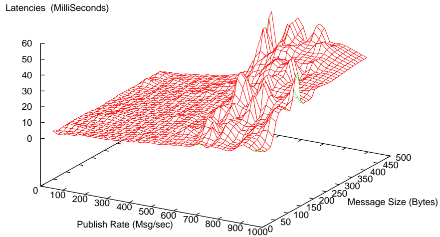
Subscriber 1 server hop from publisher - Matching 50%
