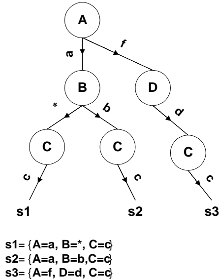
Figure 4.5: The profile graph - An example.
