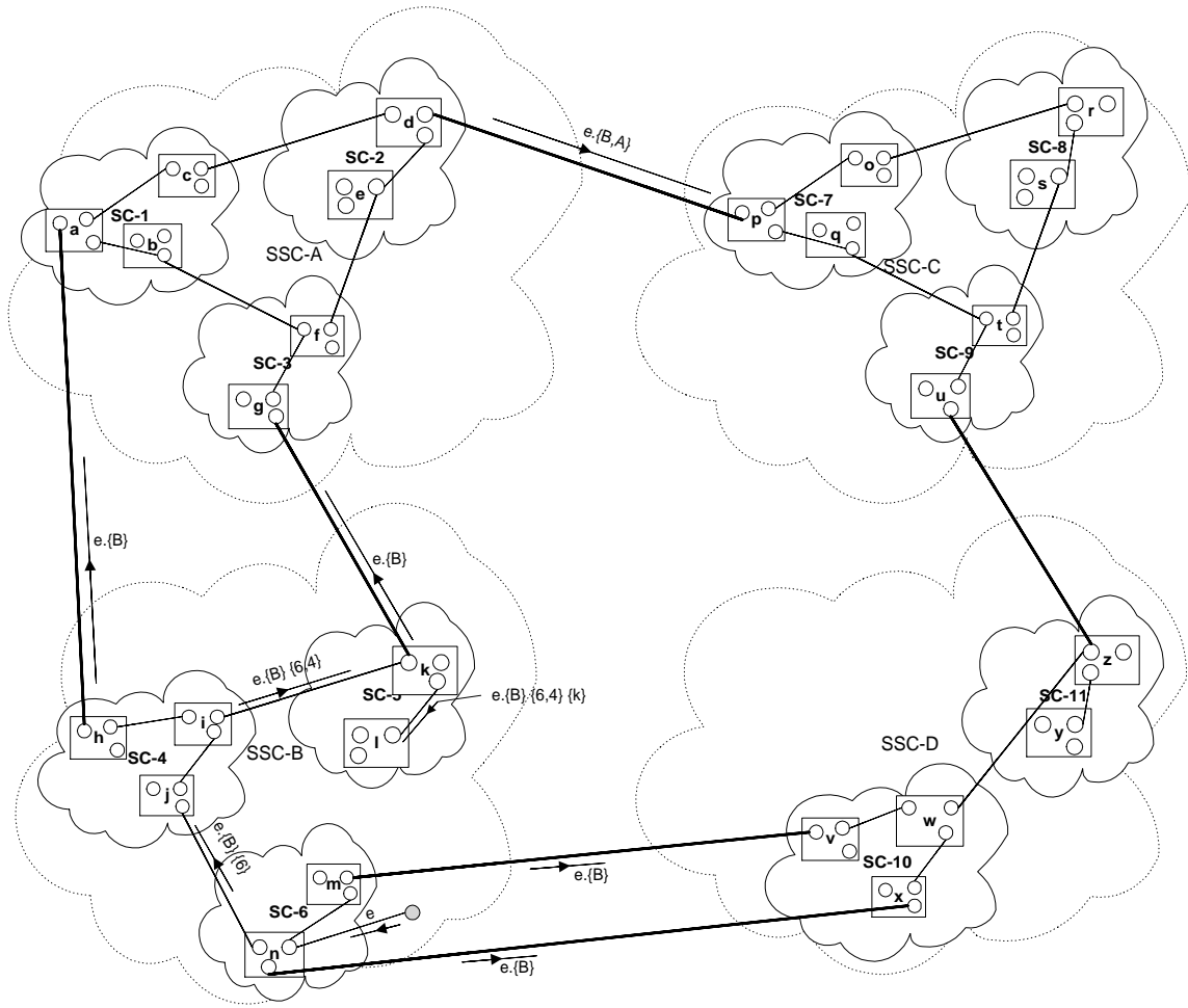
Figure 4.8: Routing events
