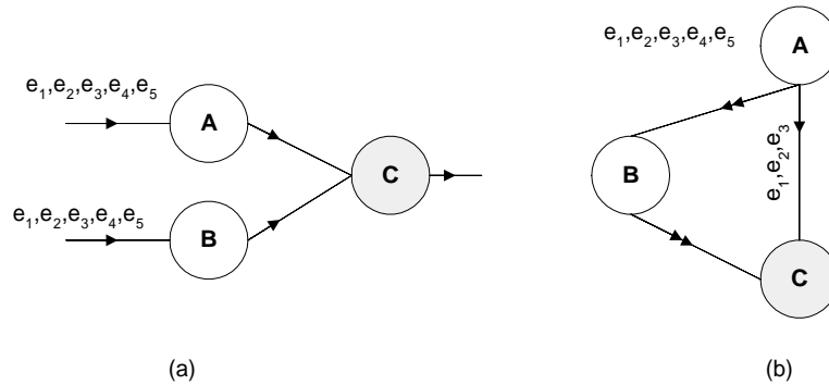
Figure 4.9: Duplicate detection of events
