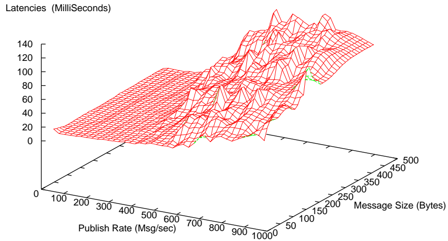
Subscriber 4 server hops from publisher - Matching 50%
