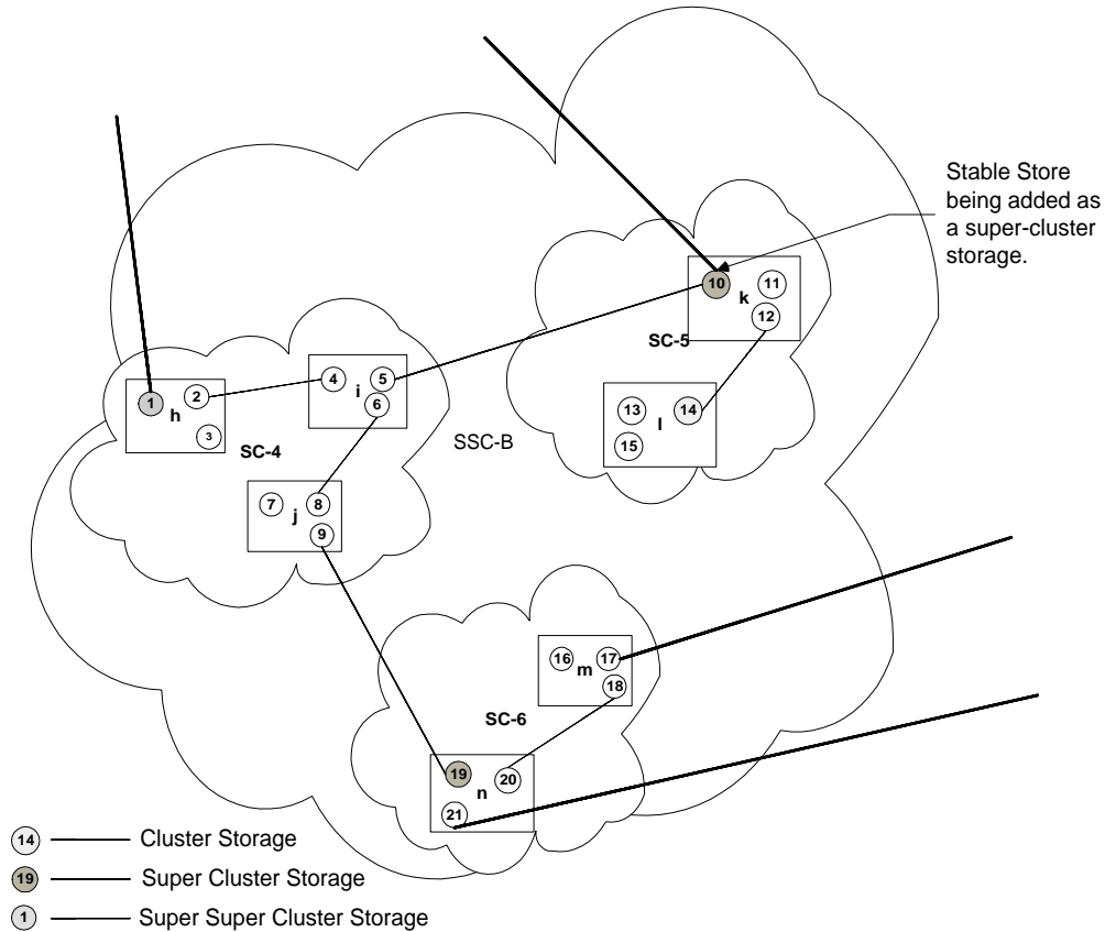
Figure 6.6: Adding stable stores
