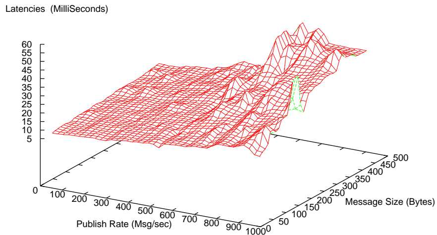
Subscriber 4 server hops from publisher - Matching 10%
