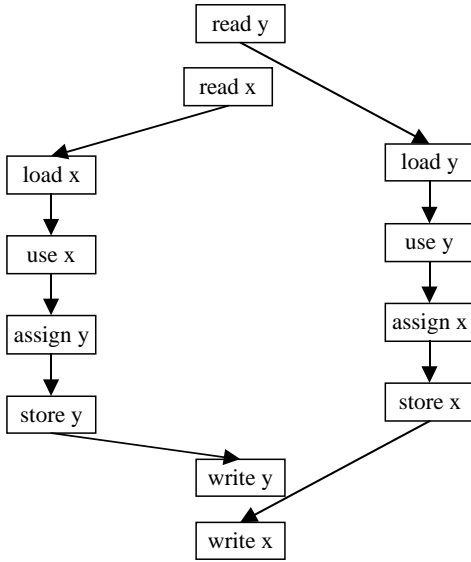
Figure 2: Actions and orderings for Figure 1 without prescient stores (with prescient stores, delete orderings from assign actions to store actions)
