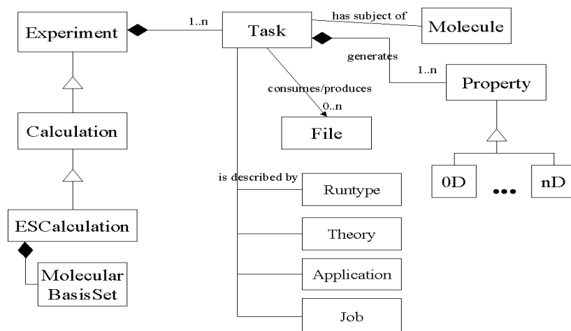
Figure 5. Simplified Ecce object model
