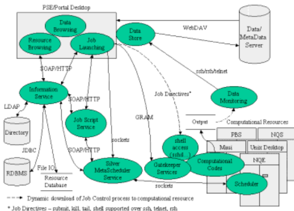
Figure 4. Operational view of planned architecture
