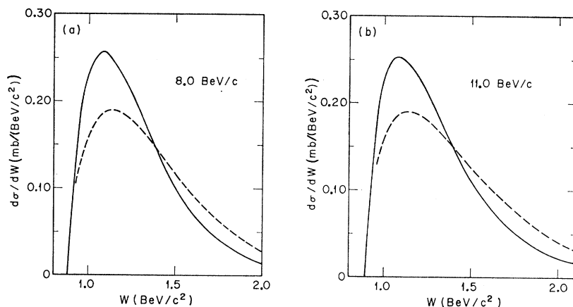
FIG. 2. Comparison of \pi\rho mass distributions calculated from pion Regge-pole-exchange model (solid line) and elementary pion-exchange Deck-type model (dashed line) for the reaction \pi N \rightarrow \pi\rho N at incident pion momenta: (a) 8.0 BeV/c and (b) 11.0 BeV/c. W is the invariant mass of the \pi\nu system.
